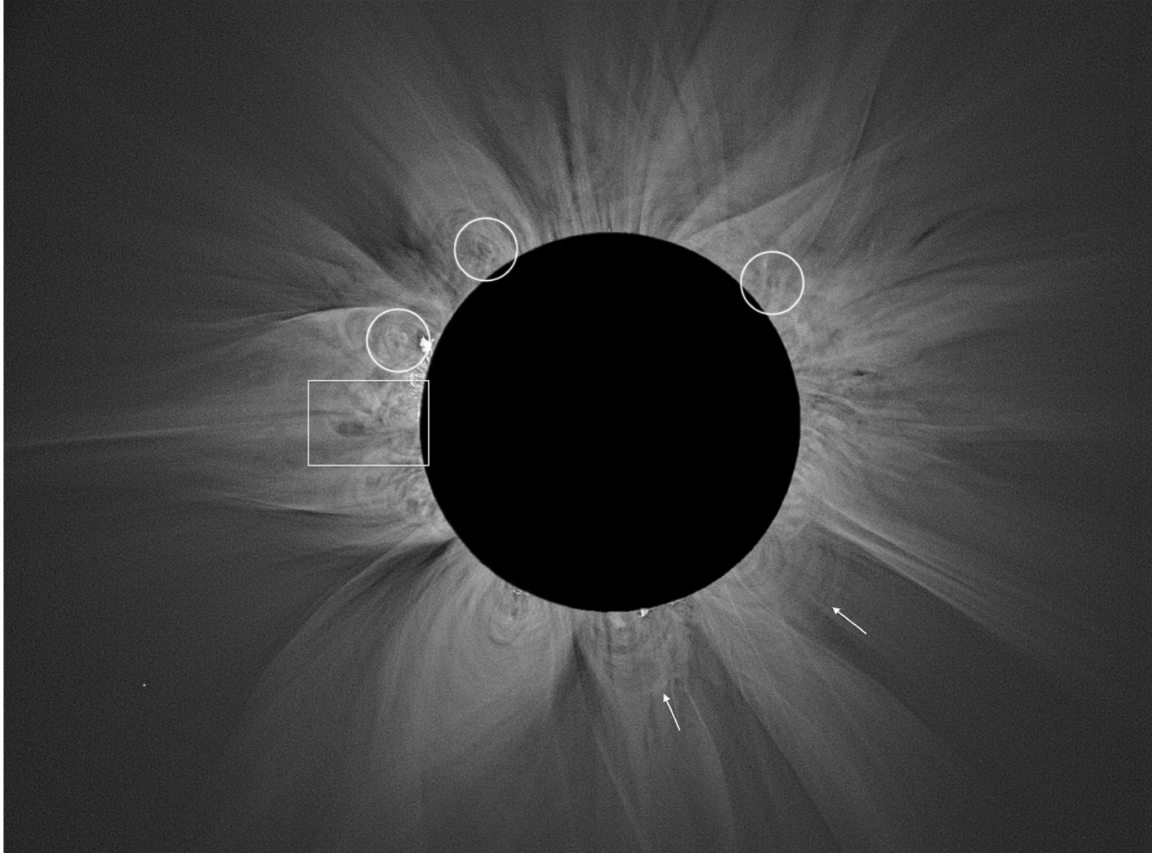
Figure 4. from Discovery of a New Class of Coronal Structures in White Light Eclipse Images Druckmüller, Habbal, & Morgan 2014 ApJ 785 14 doi:10.1088/0004-637X/785/1/14 https://dx.doi.org/10.1088/0004-637X/785/1/14 © 2014. The American Astronomical Society. All rights reserved.
