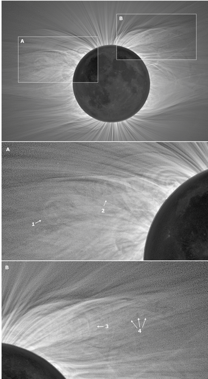
Figure 2. from Discovery of a New Class of Coronal Structures in White Light Eclipse Images Druckmüller, Habbal, & Morgan 2014 ApJ 785 14 doi:10.1088/0004-637X/785/1/14 https://dx.doi.org/10.1088/0004-637X/785/1/14 © 2014. The American Astronomical Society. All rights reserved.
