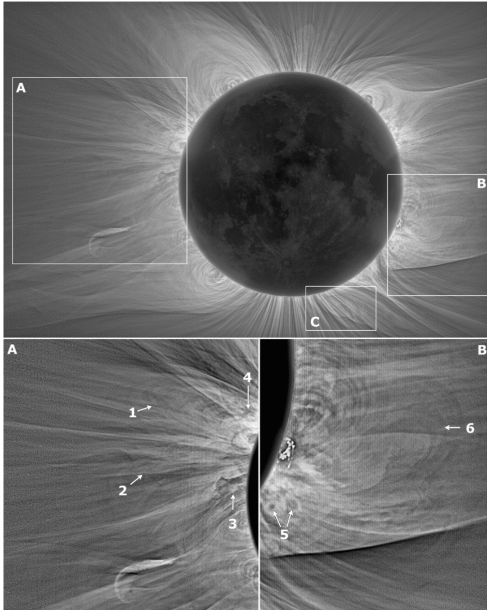
Figure 1. from Discovery of a New Class of Coronal Structures in White Light Eclipse Images Druckmüller, Habbal, & Morgan 2014 ApJ 785 14 doi:10.1088/0004-637X/785/1/14 https://dx.doi.org/10.1088/0004-637X/785/1/14 © 2014. The American Astronomical Society. All rights reserved.
