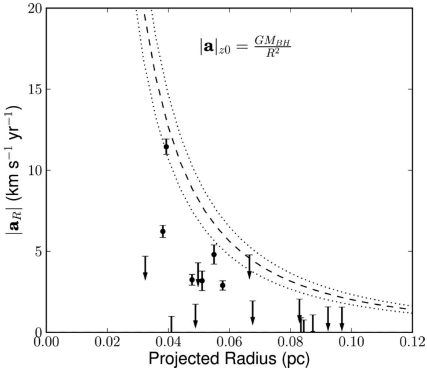
Figure 8. from Properties of the Remnant Clockwise Disk of Young Stars in the Galactic Center Yelda et al. 2014 ApJ 783 131 doi:10.1088/0004-637X/783/2/131 https://dx.doi.org/10.1088/0004-637X/783/2/131 © 2014. The American Astronomical Society. All rights reserved.
