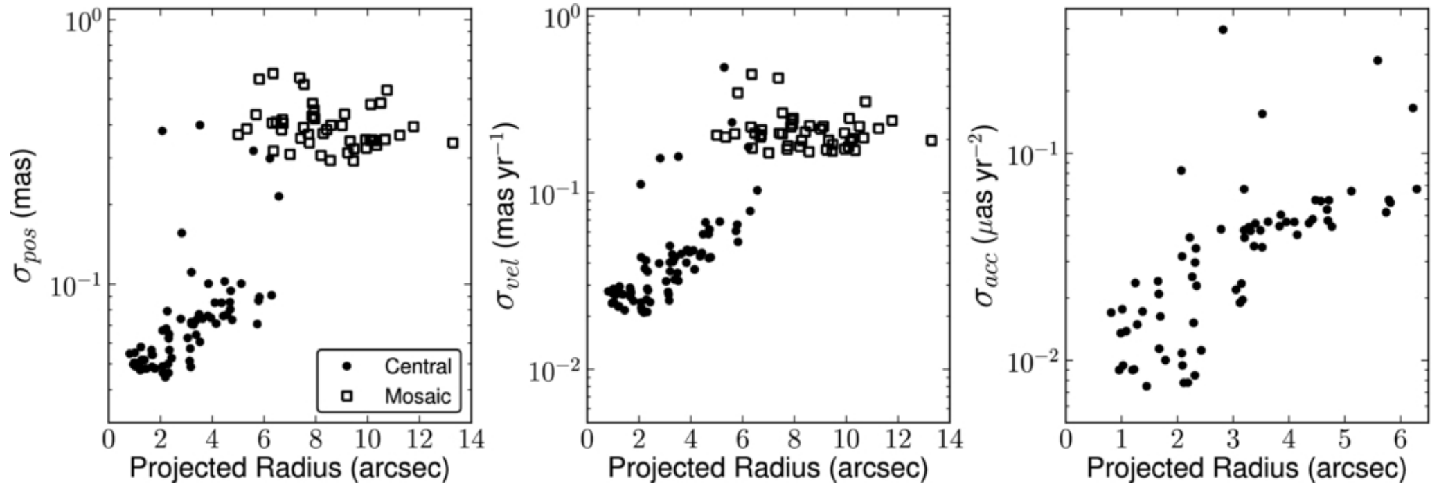
Figure 5. from Properties of the Remnant Clockwise Disk of Young Stars in the Galactic Center Yelda et al. 2014 ApJ 783 131 doi:10.1088/0004-637X/783/2/131 https://dx.doi.org/10.1088/0004-637X/783/2/131 © 2014. The American Astronomical Society. All rights reserved.
