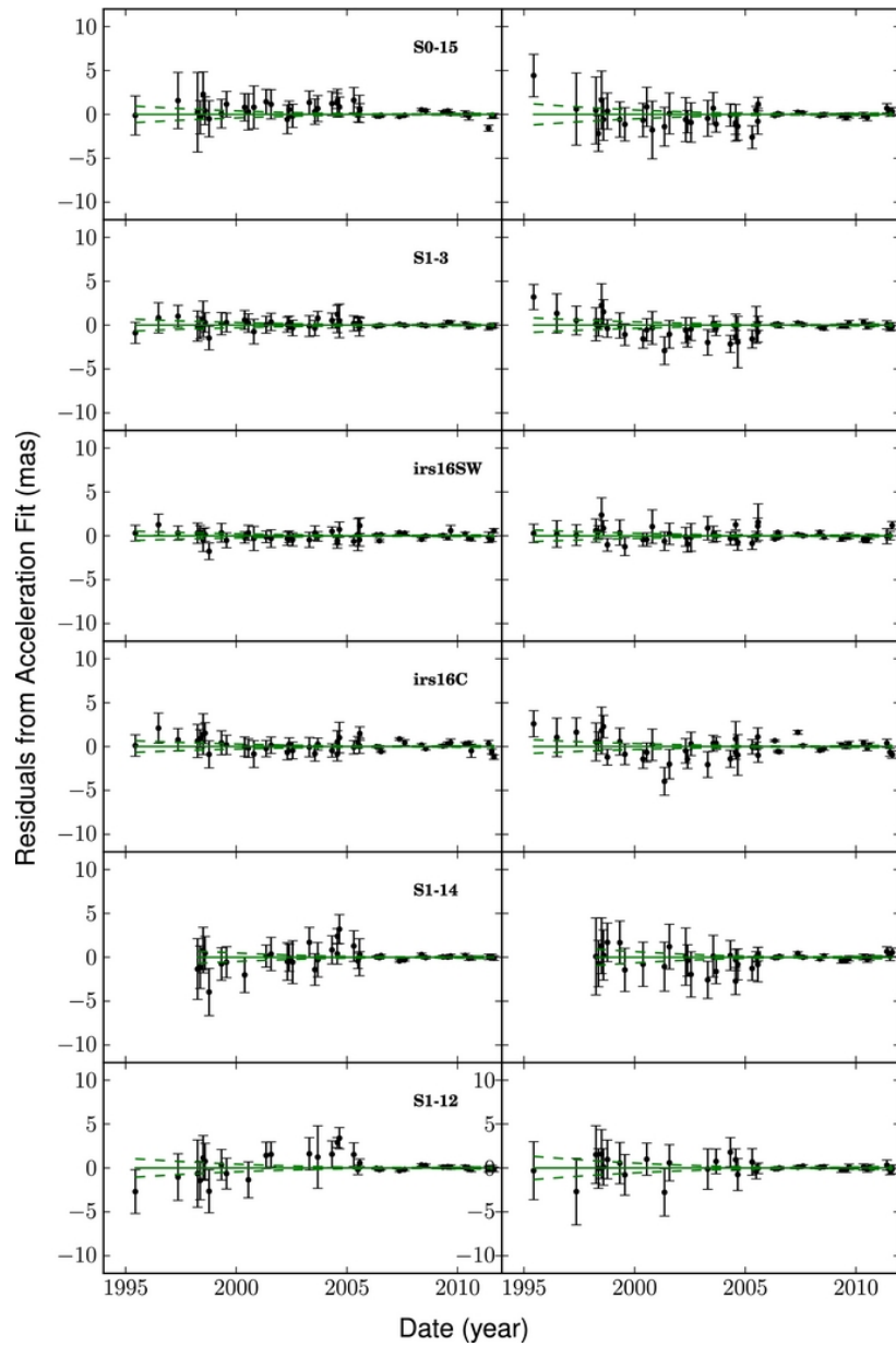
Figure 4. from Properties of the Remnant Clockwise Disk of Young Stars in the Galactic Center Yelda et al. 2014 ApJ 783 131 doi:10.1088/0004-637X/783/2/131 https://dx.doi.org/10.1088/0004-637X/783/2/131 © 2014. The American Astronomical Society. All rights reserved.
