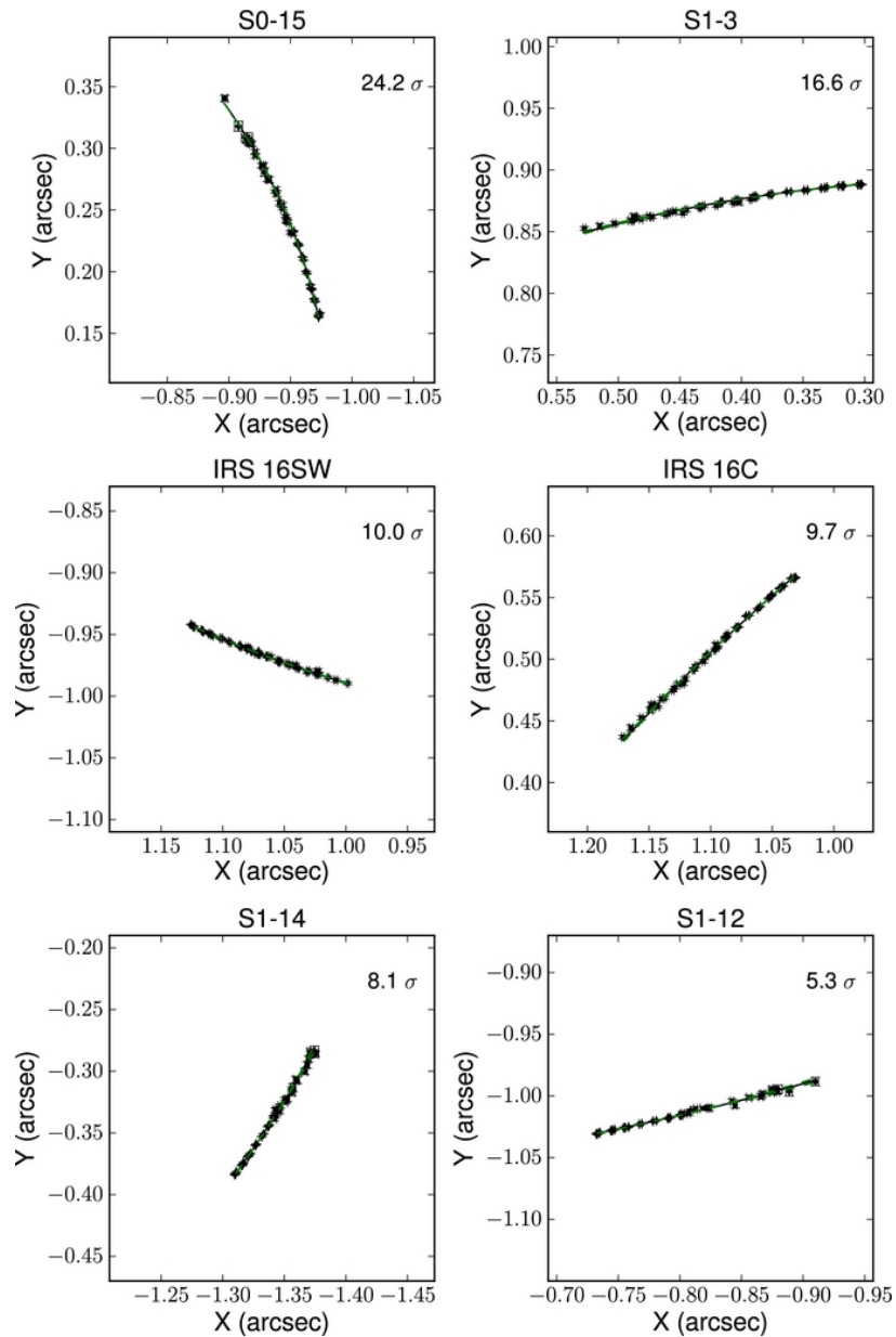
Figure 3. from Properties of the Remnant Clockwise Disk of Young Stars in the Galactic Center Yelda et al. 2014 ApJ 783 131 doi:10.1088/0004-637X/783/2/131 https://dx.doi.org/10.1088/0004-637X/783/2/131 © 2014. The American Astronomical Society. All rights reserved.
