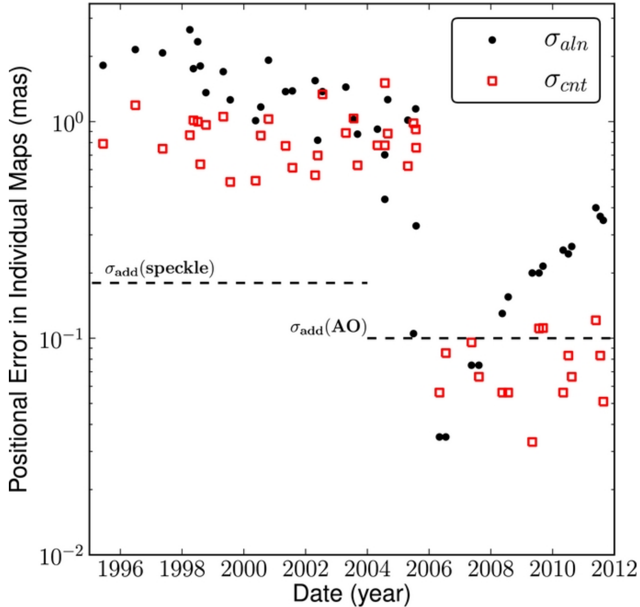
Figure 2. from Properties of the Remnant Clockwise Disk of Young Stars in the Galactic Center Yelda et al. 2014 ApJ 783 131 doi:10.1088/0004-637X/783/2/131 https://dx.doi.org/10.1088/0004-637X/783/2/131 © 2014. The American Astronomical Society. All rights reserved.
