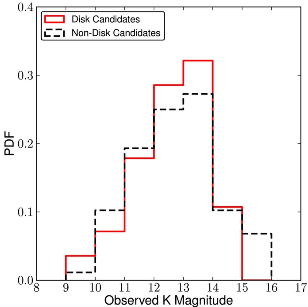
Figure 19. from Properties of the Remnant Clockwise Disk of Young Stars in the Galactic Center Yelda et al. 2014 ApJ 783 131 doi:10.1088/0004-637X/783/2/131 https://dx.doi.org/10.1088/0004-637X/783/2/131 © 2014. The American Astronomical Society. All rights reserved.
