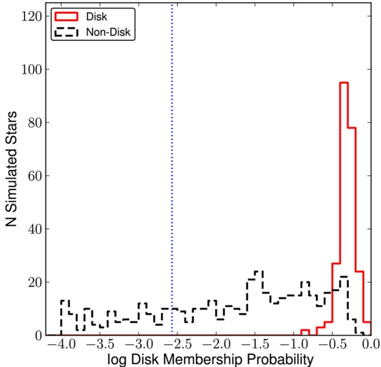
Figure 18. from Properties of the Remnant Clockwise Disk of Young Stars in the Galactic Center Yelda et al. 2014 ApJ 783 131 doi:10.1088/0004-637X/783/2/131 https://dx.doi.org/10.1088/0004-637X/783/2/131 © 2014. The American Astronomical Society. All rights reserved.
