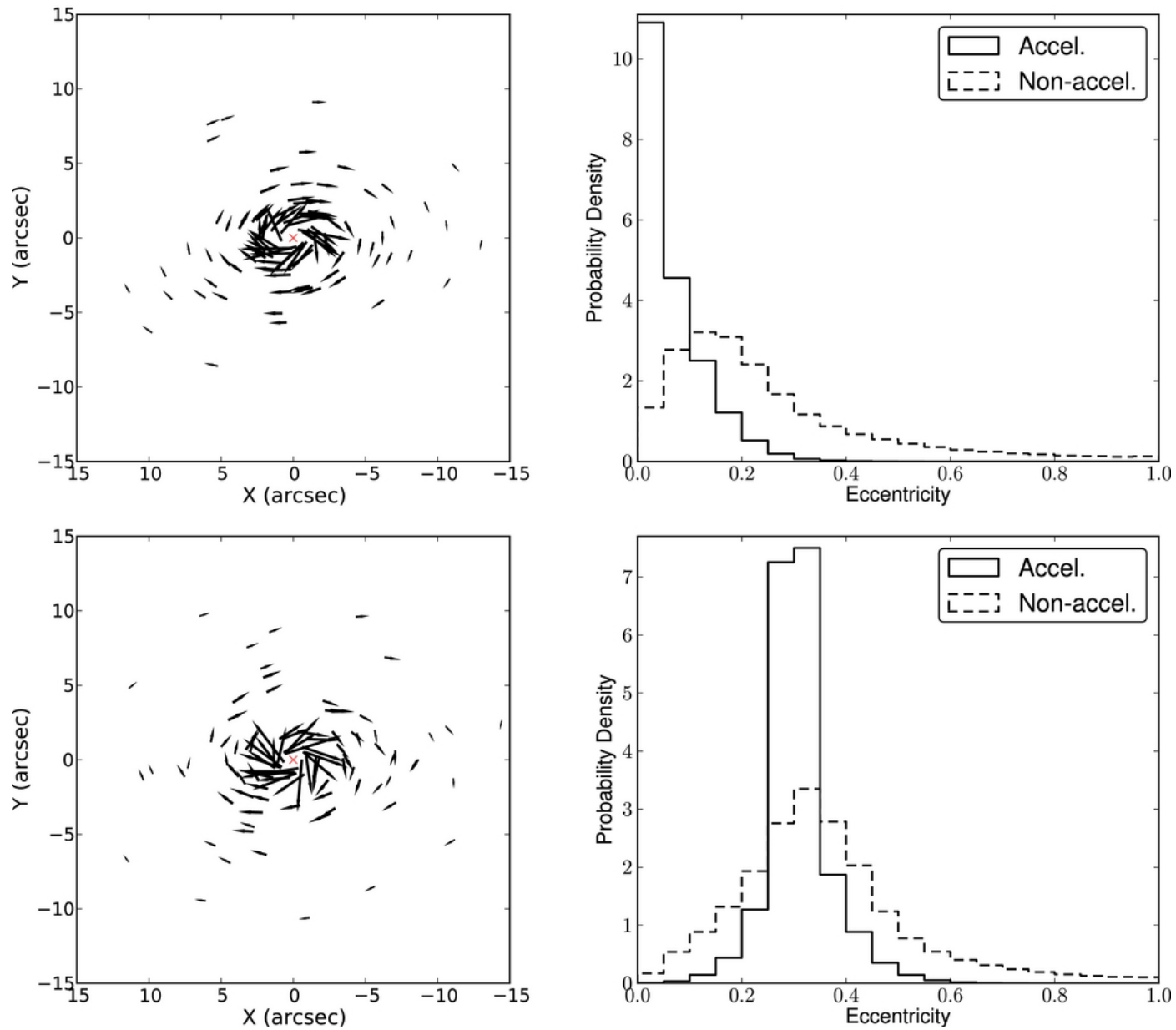
Figure 15. from Properties of the Remnant Clockwise Disk of Young Stars in the Galactic Center Yelda et al. 2014 ApJ 783 131 doi:10.1088/0004-637X/783/2/131 https://dx.doi.org/10.1088/0004-637X/783/2/131 © 2014. The American Astronomical Society. All rights reserved.
