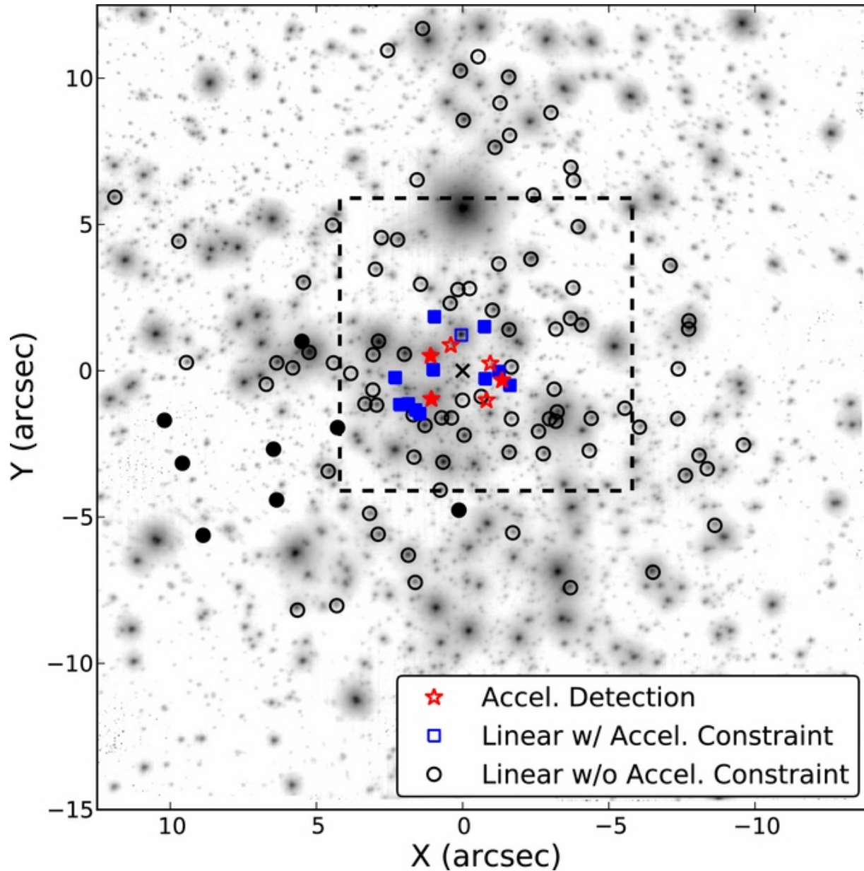
Figure 1. from Properties of the Remnant Clockwise Disk of Young Stars in the Galactic Center Yelda et al. 2014 ApJ 783 131 doi:10.1088/0004-637X/783/2/131 https://dx.doi.org/10.1088/0004-637X/783/2/131 © 2014. The American Astronomical Society. All rights reserved.
