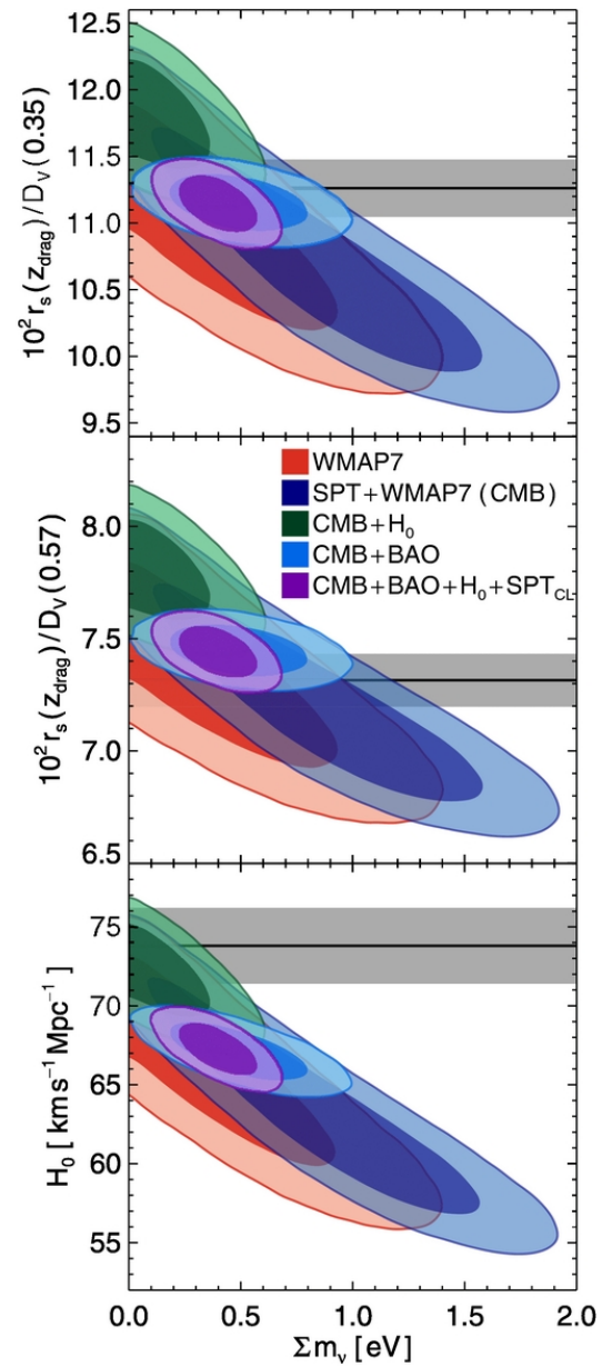
Figure 9. from Constraints on Cosmology from the Cosmic Microwave Background Power Spectrum of the 2500 deg 2 SPT-SZ Survey Hou et al. 2014 ApJ 782 74 doi:10.1088/0004-637X/782/2/74 https://dx.doi.org/10.1088/0004-637X/782/2/74 © 2014. The American Astronomical Society. All rights reserved.
