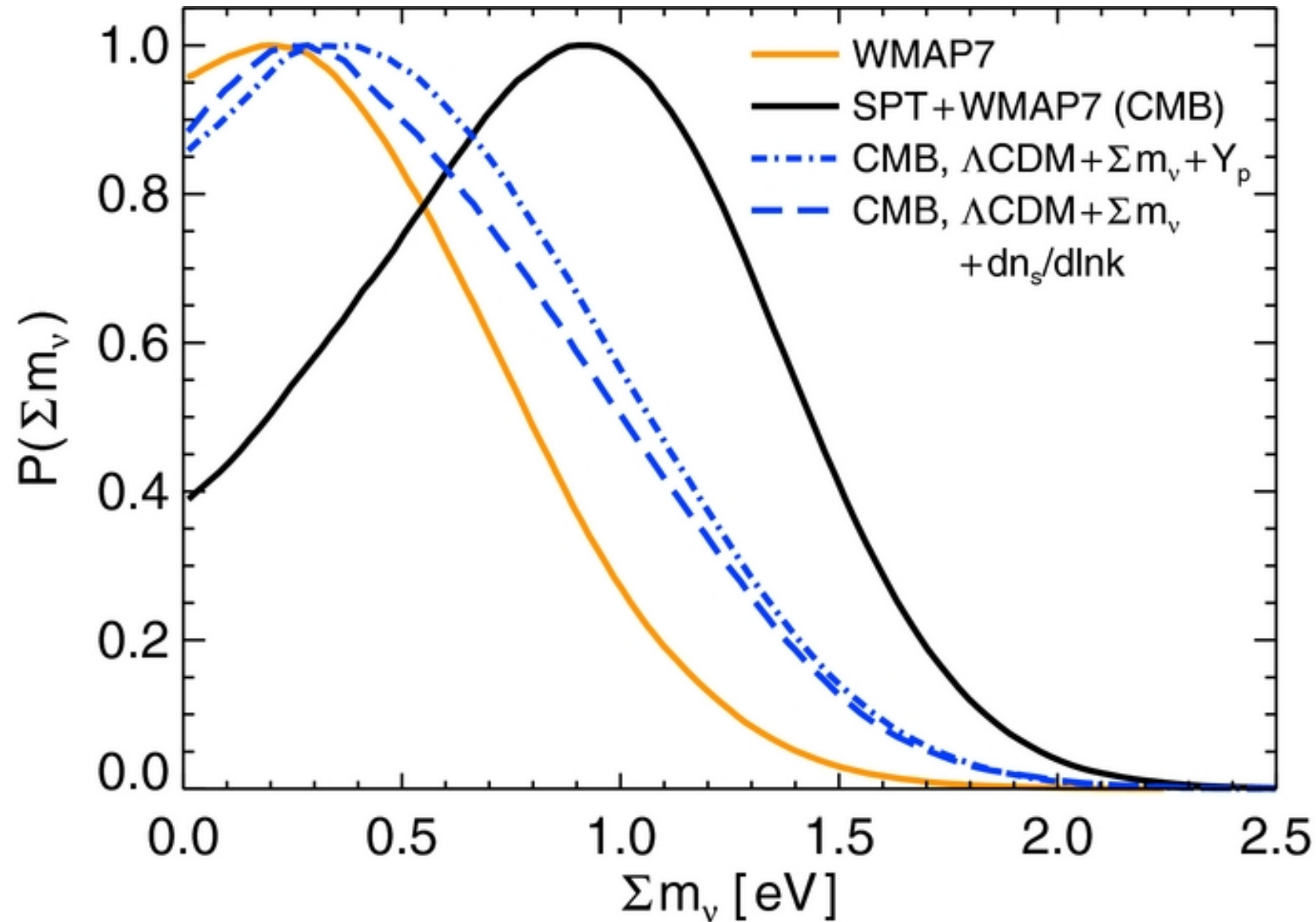
Figure 8. from Constraints on Cosmology from the Cosmic Microwave Background Power Spectrum of the 2500 deg 2 SPT-SZ Survey Hou et al. 2014 ApJ 782 74 doi:10.1088/0004-637X/782/2/74 https://dx.doi.org/10.1088/0004-637X/782/2/74 © 2014. The American Astronomical Society. All rights reserved.
