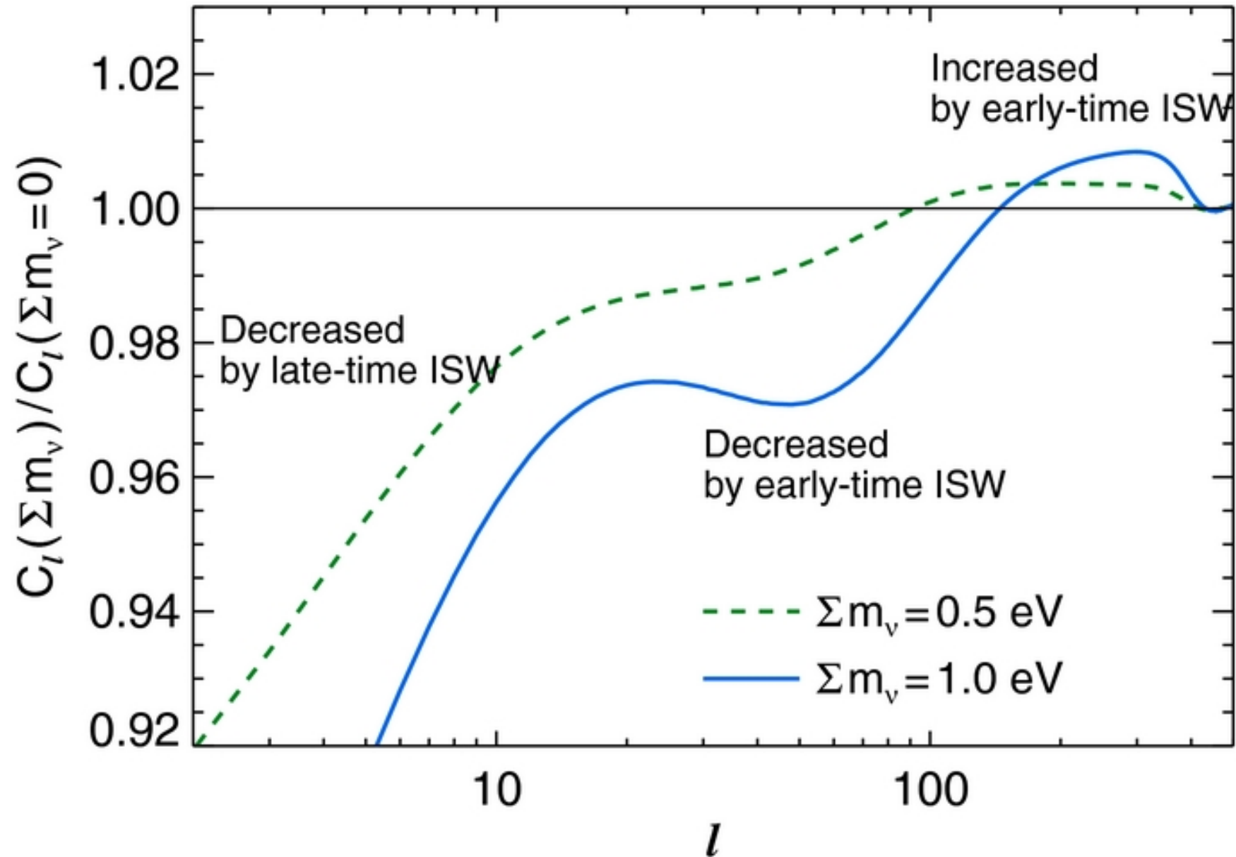
Figure 6. from Constraints on Cosmology from the Cosmic Microwave Background Power Spectrum of the 2500 deg 2 SPT-SZ Survey Hou et al. 2014 ApJ 782 74 doi:10.1088/0004-637X/782/2/74 https://dx.doi.org/10.1088/0004-637X/782/2/74 © 2014. The American Astronomical Society. All rights reserved.
