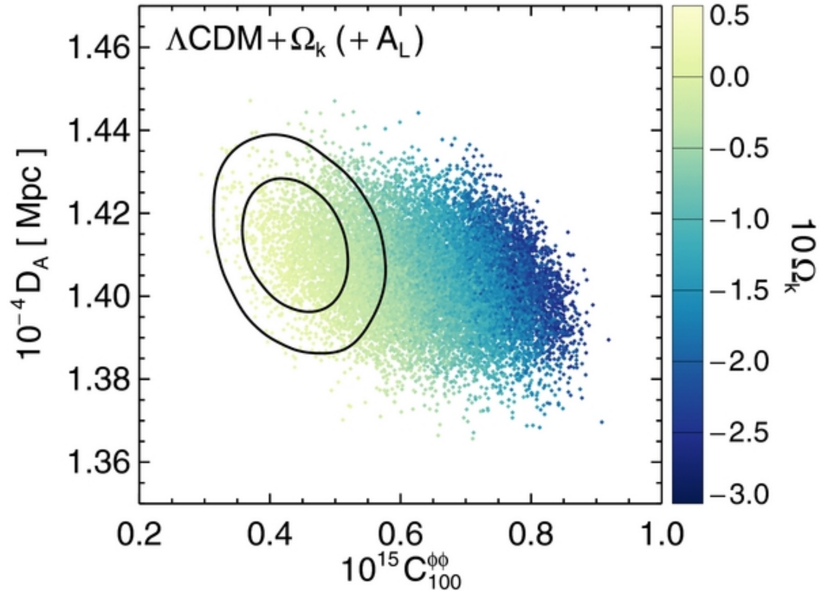
Figure 5. from Constraints on Cosmology from the Cosmic Microwave Background Power Spectrum of the 2500 deg 2 SPT-SZ Survey Hou et al. 2014 ApJ 782 74 doi:10.1088/0004-637X/782/2/74 https://dx.doi.org/10.1088/0004-637X/782/2/74 © 2014. The American Astronomical Society. All rights reserved.
