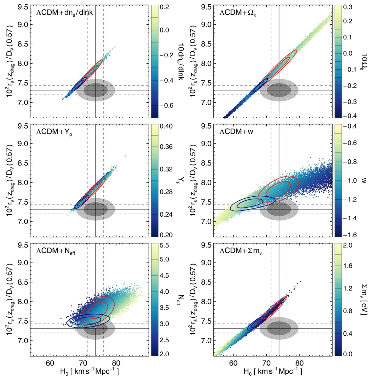
Figure 4. from Constraints on Cosmology from the Cosmic Microwave Background Power Spectrum of the 2500 deg 2 SPT-SZ Survey Hou et al. 2014 ApJ 782 74 doi:10.1088/0004-637X/782/2/74 https://dx.doi.org/10.1088/0004-637X/782/2/74 © 2014. The American Astronomical Society. All rights reserved.
