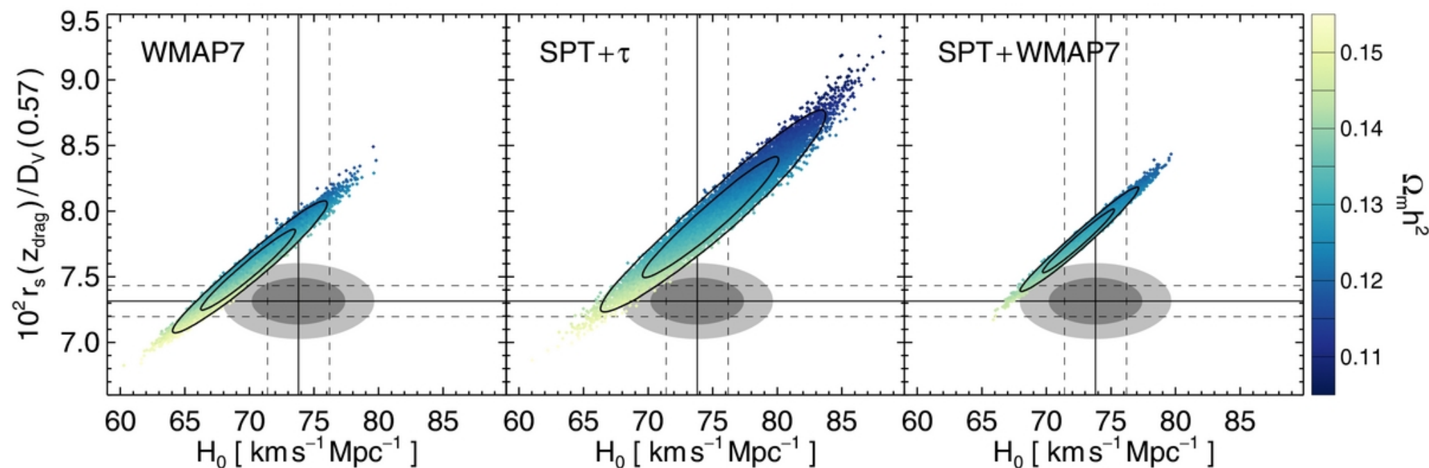
Figure 3. from Constraints on Cosmology from the Cosmic Microwave Background Power Spectrum of the 2500 deg 2 SPT-SZ Survey Hou et al. 2014 ApJ 782 74 doi:10.1088/0004-637X/782/2/74 https://dx.doi.org/10.1088/0004-637X/782/2/74 © 2014. The American Astronomical Society. All rights reserved.
