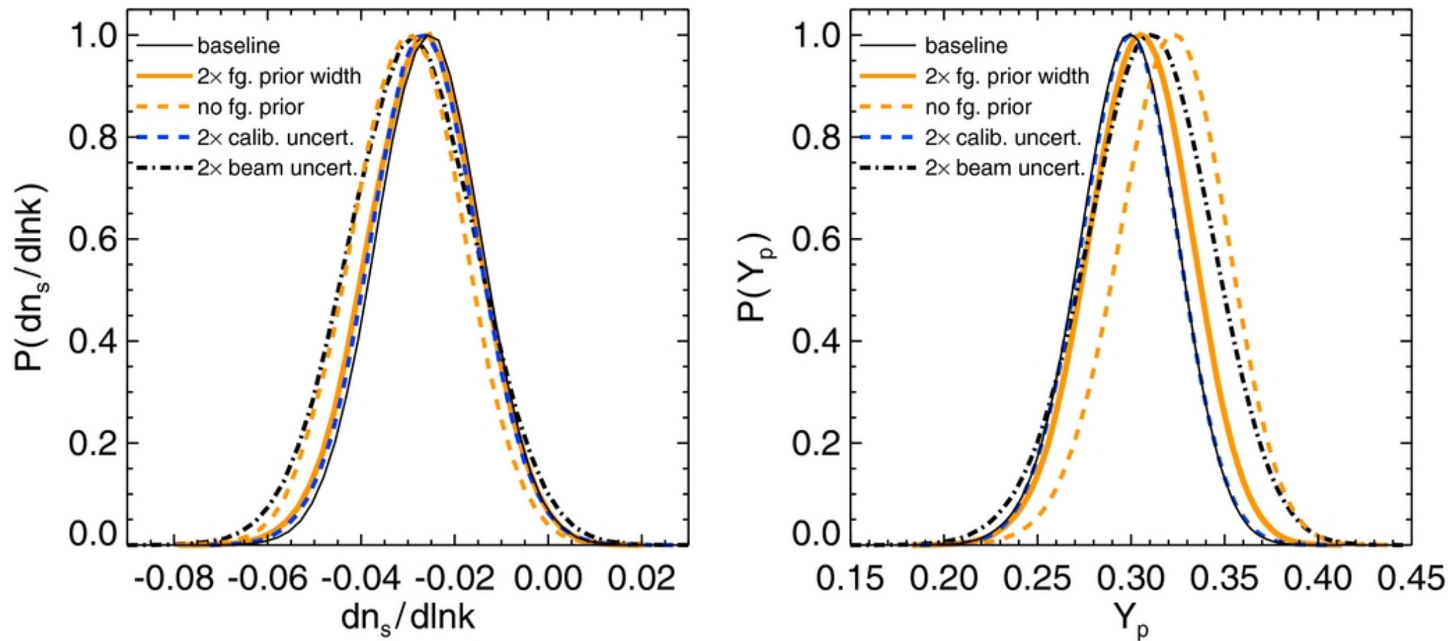
Figure 20. from Constraints on Cosmology from the Cosmic Microwave Background Power Spectrum of the 2500 deg 2 SPT-SZ Survey Hou et al. 2014 ApJ 782 74 doi:10.1088/0004-637X/782/2/74 https://dx.doi.org/10.1088/0004-637X/782/2/74 © 2014. The American Astronomical Society. All rights reserved.
