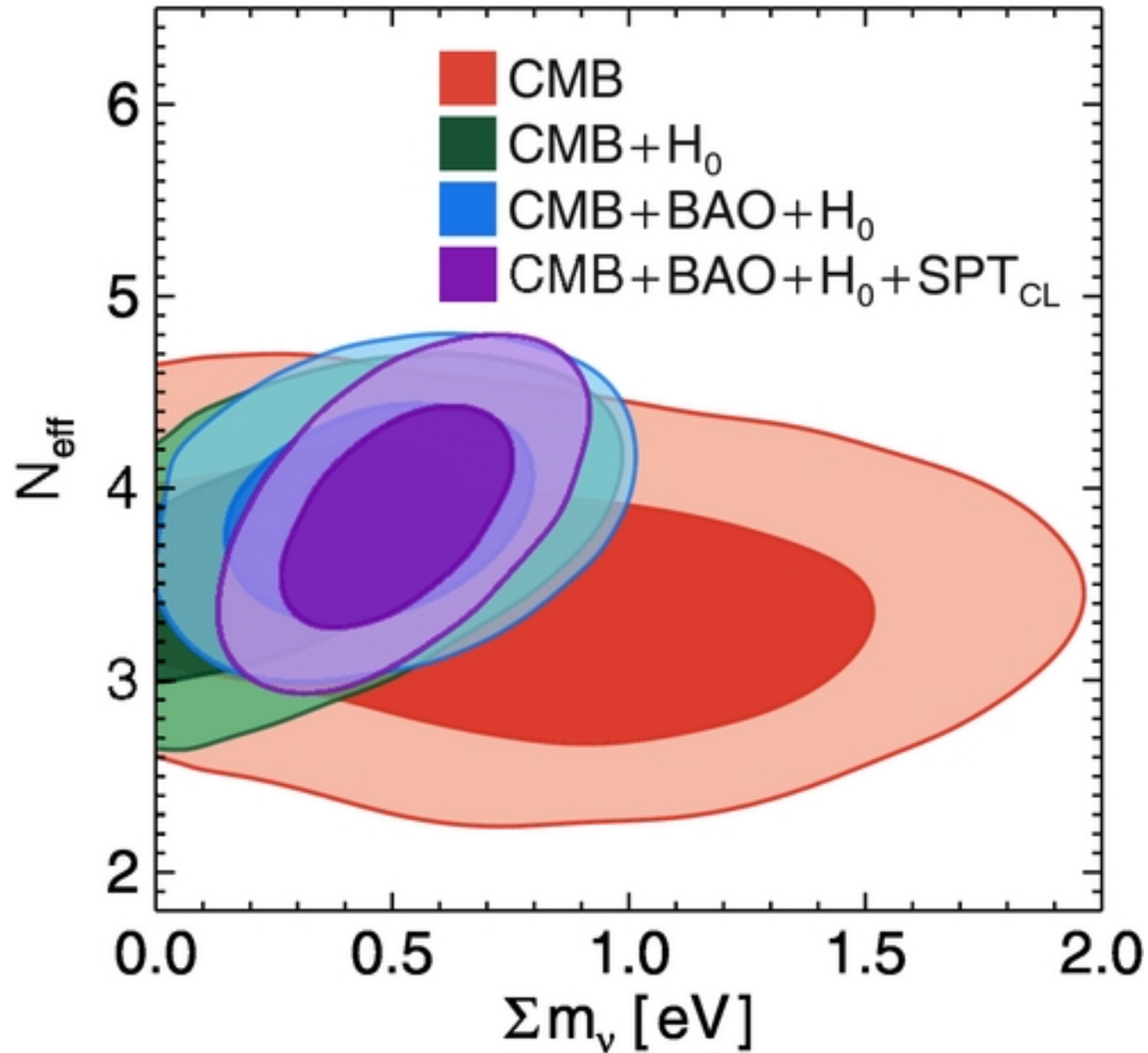
Figure 19. from Constraints on Cosmology from the Cosmic Microwave Background Power Spectrum of the 2500 deg 2 SPT-SZ Survey Hou et al. 2014 ApJ 782 74 doi:10.1088/0004-637X/782/2/74 https://dx.doi.org/10.1088/0004-637X/782/2/74 © 2014. The American Astronomical Society. All rights reserved.
