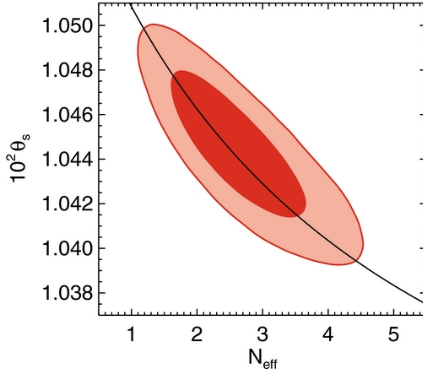
Figure 16. from Constraints on Cosmology from the Cosmic Microwave Background Power Spectrum of the 2500 deg 2 SPT-SZ Survey Hou et al. 2014 ApJ 782 74 doi:10.1088/0004-637X/782/2/74 https://dx.doi.org/10.1088/0004-637X/782/2/74 © 2014. The American Astronomical Society. All rights reserved.
