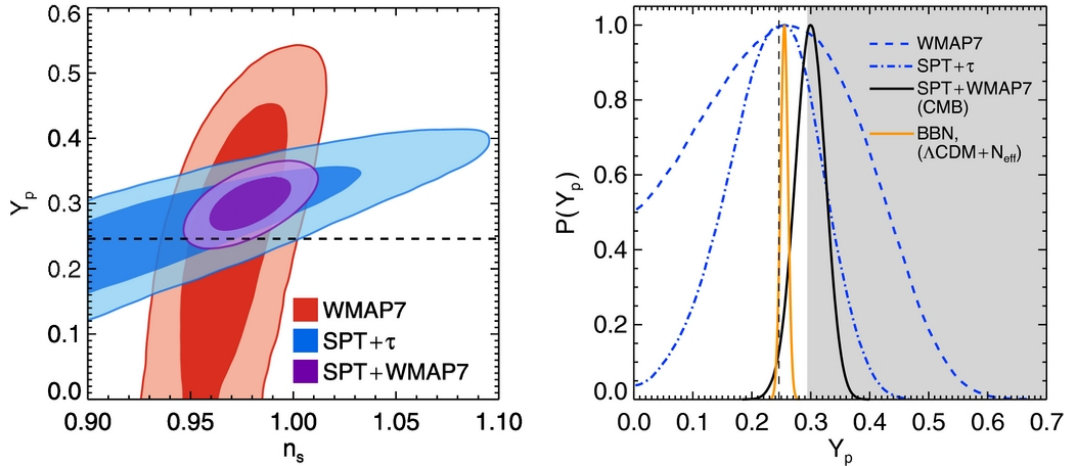
Figure 15. from Constraints on Cosmology from the Cosmic Microwave Background Power Spectrum of the 2500 deg 2 SPT-SZ Survey Hou et al. 2014 ApJ 782 74 doi:10.1088/0004-637X/782/2/74 https://dx.doi.org/10.1088/0004-637X/782/2/74 © 2014. The American Astronomical Society. All rights reserved.
