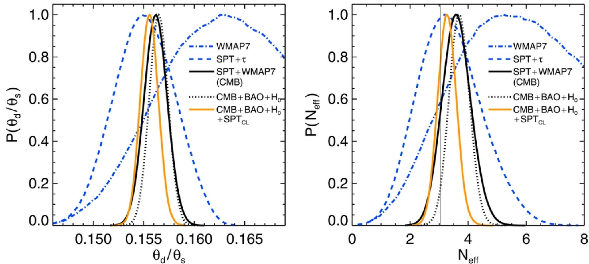
Figure 14. from Constraints on Cosmology from the Cosmic Microwave Background Power Spectrum of the 2500 deg 2 SPT-SZ Survey Hou et al. 2014 ApJ 782 74 doi:10.1088/0004-637X/782/2/74 https://dx.doi.org/10.1088/0004-637X/782/2/74 © 2014. The American Astronomical Society. All rights reserved.
