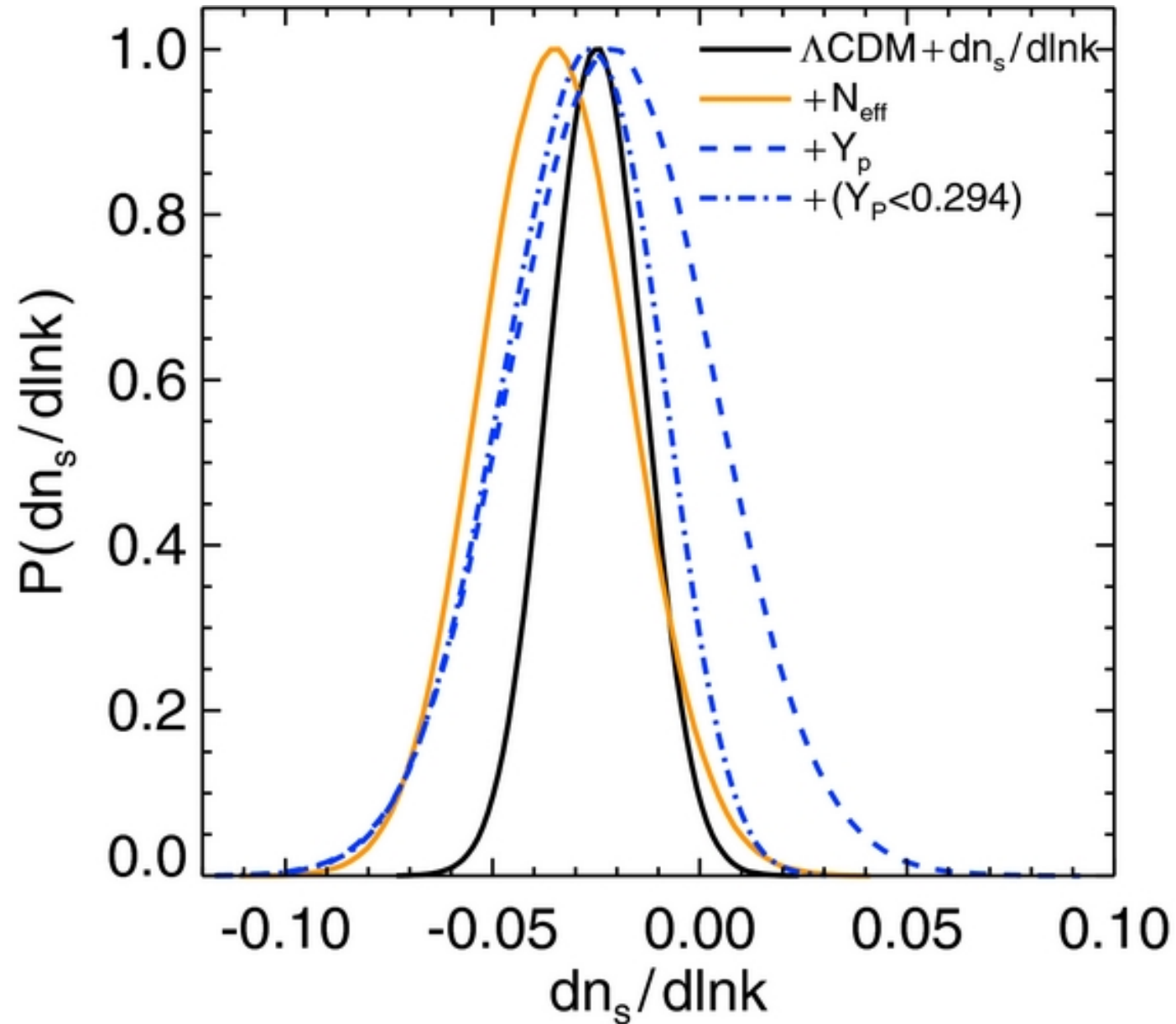
Figure 13. from Constraints on Cosmology from the Cosmic Microwave Background Power Spectrum of the 2500 deg 2 SPT-SZ Survey Hou et al. 2014 ApJ 782 74 doi:10.1088/0004-637X/782/2/74 https://dx.doi.org/10.1088/0004-637X/782/2/74 © 2014. The American Astronomical Society. All rights reserved.
