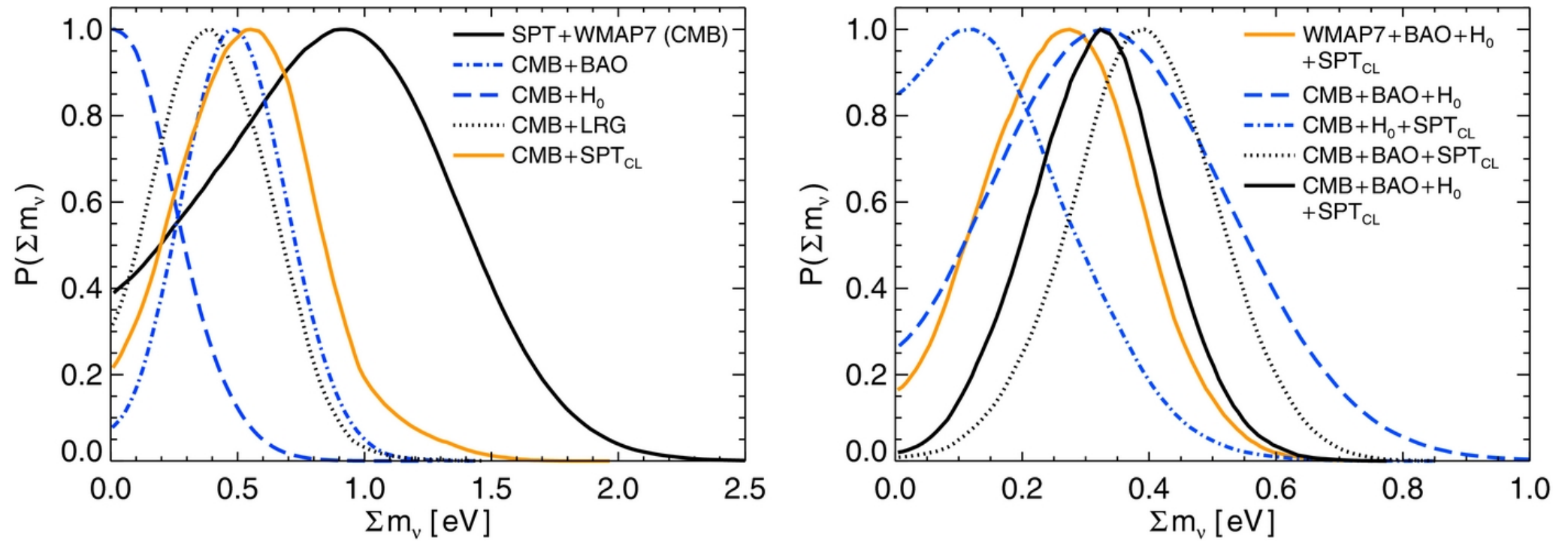
Figure 10. from Constraints on Cosmology from the Cosmic Microwave Background Power Spectrum of the 2500 deg 2 SPT-SZ Survey Hou et al. 2014 ApJ 782 74 doi:10.1088/0004-637X/782/2/74 https://dx.doi.org/10.1088/0004-637X/782/2/74 © 2014. The American Astronomical Society. All rights reserved.
