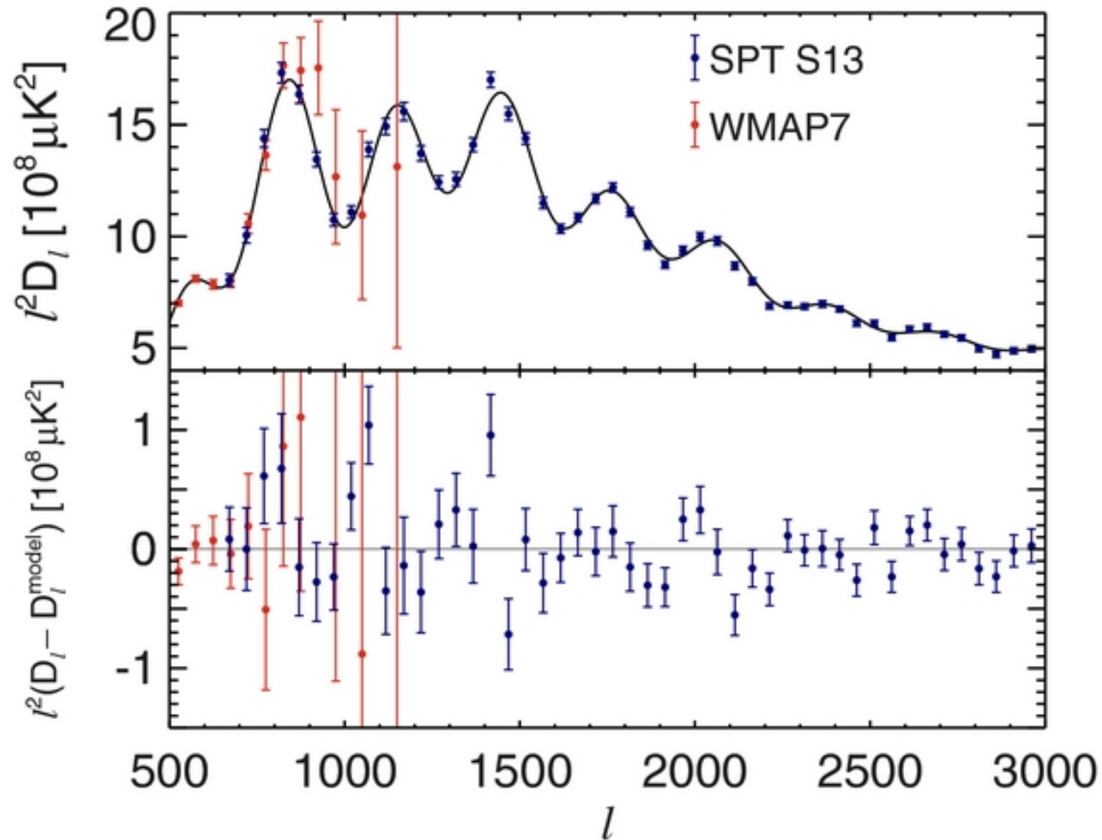
Figure 1. from Constraints on Cosmology from the Cosmic Microwave Background Power Spectrum of the 2500 deg 2 SPT-SZ Survey Hou et al. 2014 ApJ 782 74 doi:10.1088/0004-637X/782/2/74 https://dx.doi.org/10.1088/0004-637X/782/2/74 © 2014. The American Astronomical Society. All rights reserved.
