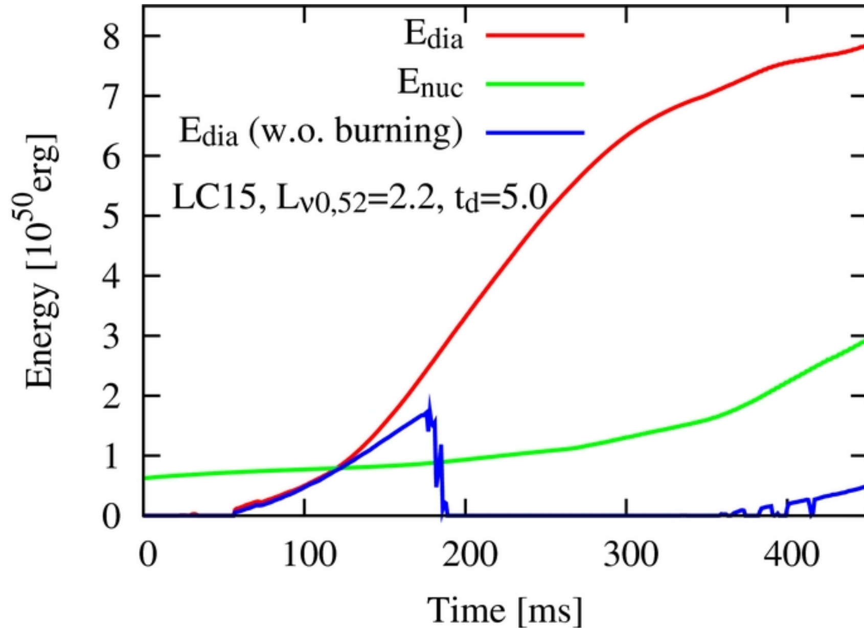
Figure 9. from Revisiting Impacts of Nuclear Burning for Reviving Weak Shocks in Neutrino-driven Supernovae Nakamura et al. 2014 ApJ 782 91 doi:10.1088/0004-637X/782/2/91 https://dx.doi.org/10.1088/0004-637X/782/2/91 © 2014. The American Astronomical Society. All rights reserved.
