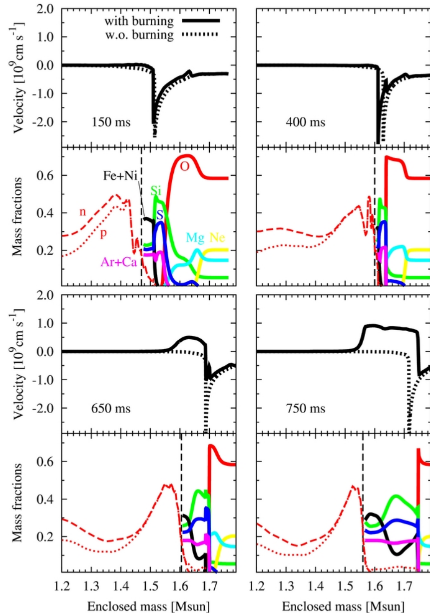
Figure 7. from Revisiting Impacts of Nuclear Burning for Reviving Weak Shocks in Neutrino-driven Supernovae Nakamura et al. 2014 ApJ 782 91 doi:10.1088/0004-637X/782/2/91 https://dx.doi.org/10.1088/0004-637X/782/2/91
