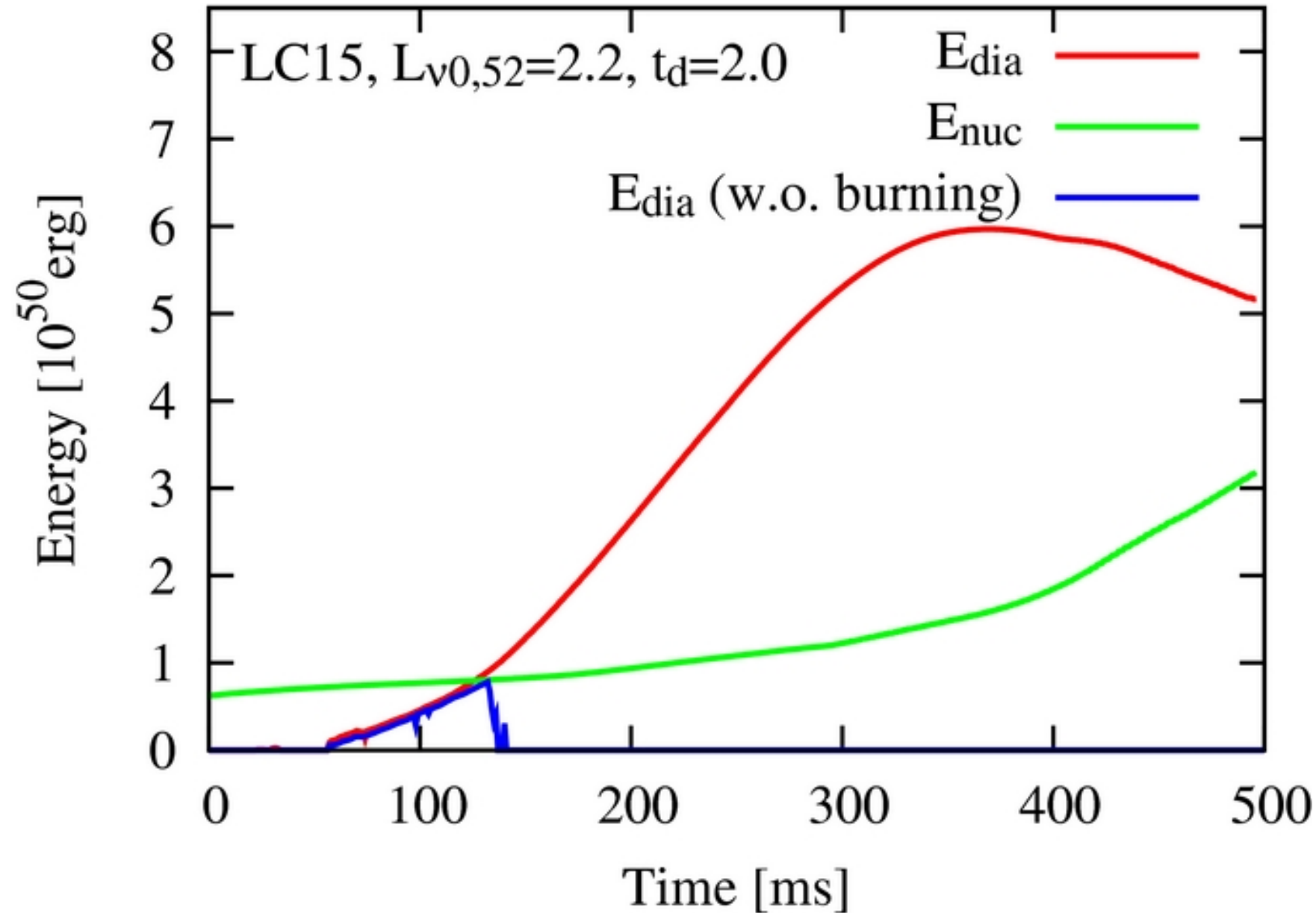
Figure 6. from Revisiting Impacts of Nuclear Burning for Reviving Weak Shocks in Neutrino-driven Supernovae Nakamura et al. 2014 ApJ 782 91 doi:10.1088/0004-637X/782/2/91 https://dx.doi.org/10.1088/0004-637X/782/2/91 © 2014. The American Astronomical Society. All rights reserved.
