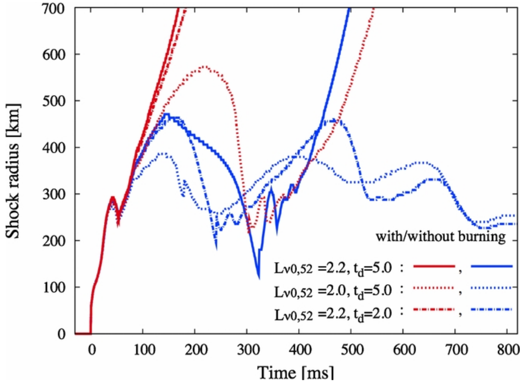
Figure 2. from Revisiting Impacts of Nuclear Burning for Reviving Weak Shocks in Neutrino-driven Supernovae Nakamura et al. 2014 ApJ 782 91 doi:10.1088/0004-637X/782/2/91 https://dx.doi.org/10.1088/0004-637X/782/2/91 © 2014. The American Astronomical Society. All rights reserved.
