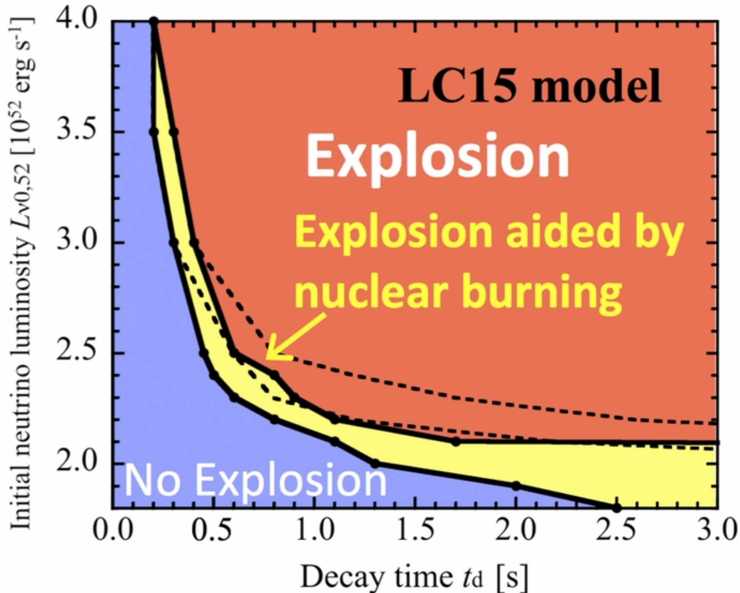
Figure 18. from Revisiting Impacts of Nuclear Burning for Reviving Weak Shocks in Neutrino-driven Supernovae Nakamura et al. 2014 ApJ 782 91 doi:10.1088/0004-637X/782/2/91 https://dx.doi.org/10.1088/0004-637X/782/2/91 © 2014. The American Astronomical Society. All rights reserved.
