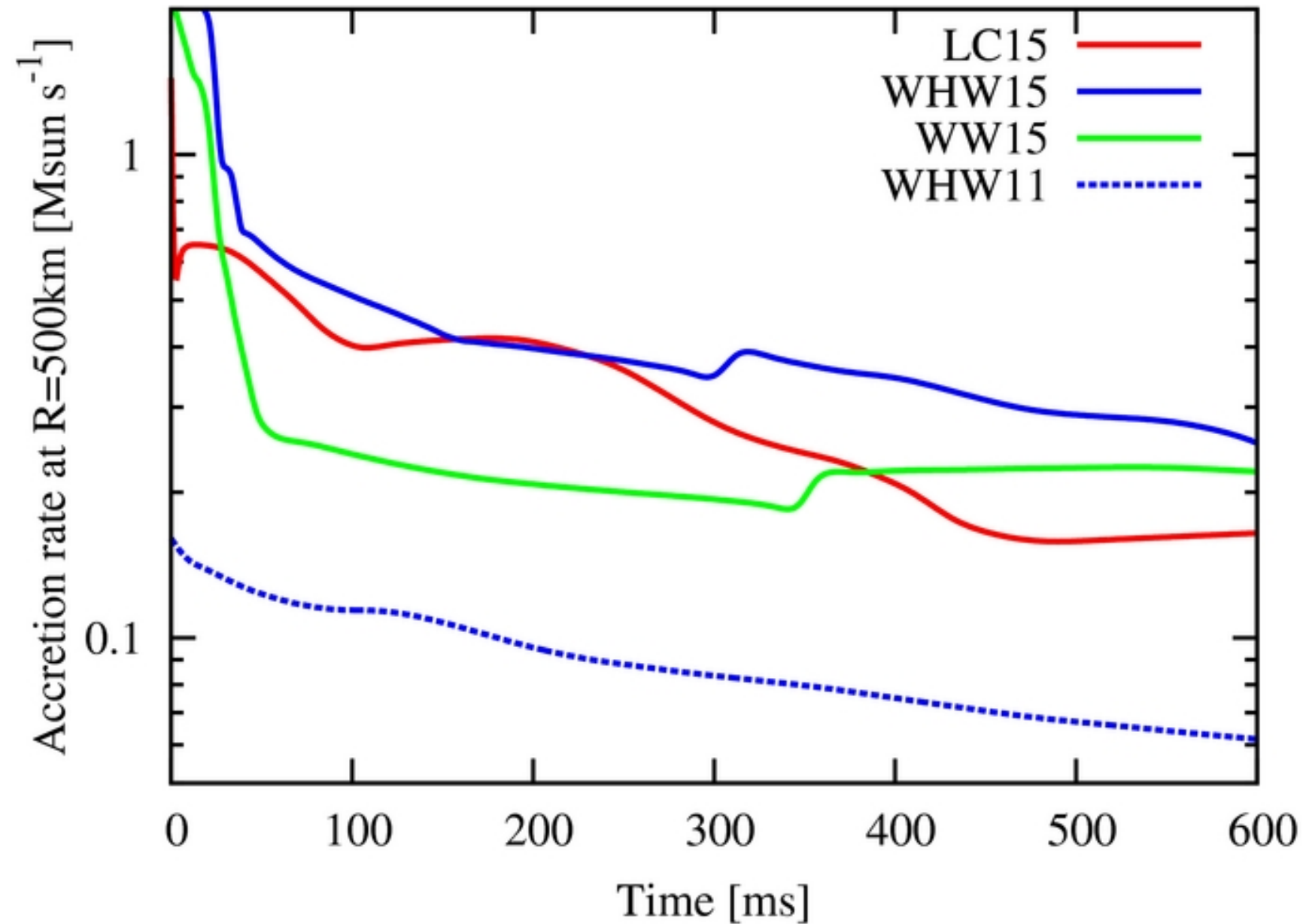
Figure 11. from Revisiting Impacts of Nuclear Burning for Reviving Weak Shocks in Neutrino-driven Supernovae Nakamura et al. 2014 ApJ 782 91 doi:10.1088/0004-637X/782/2/91 https://dx.doi.org/10.1088/0004-637X/782/2/91 © 2014. The American Astronomical Society. All rights reserved.
