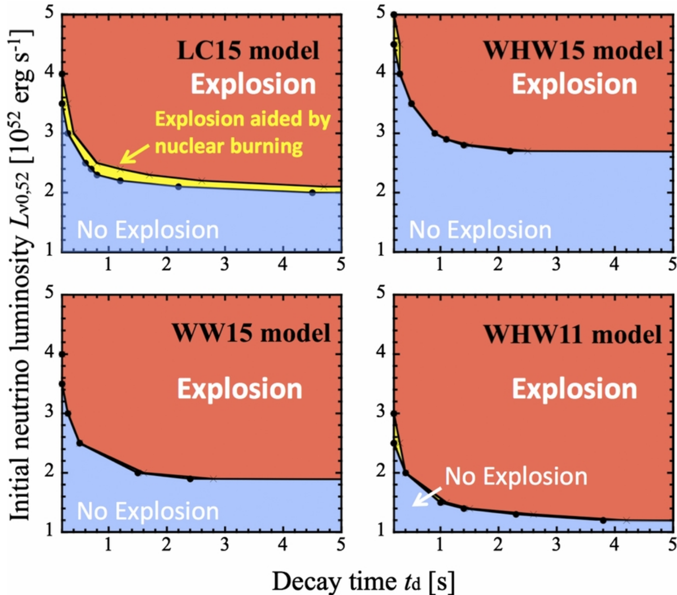
Figure 10. from Revisiting Impacts of Nuclear Burning for Reviving Weak Shocks in Neutrino-driven Supernovae Nakamura et al. 2014 ApJ 782 91 doi:10.1088/0004-637X/782/2/91 https://dx.doi.org/10.1088/0004-637X/782/2/91 © 2014. The American Astronomical Society. All rights reserved.
