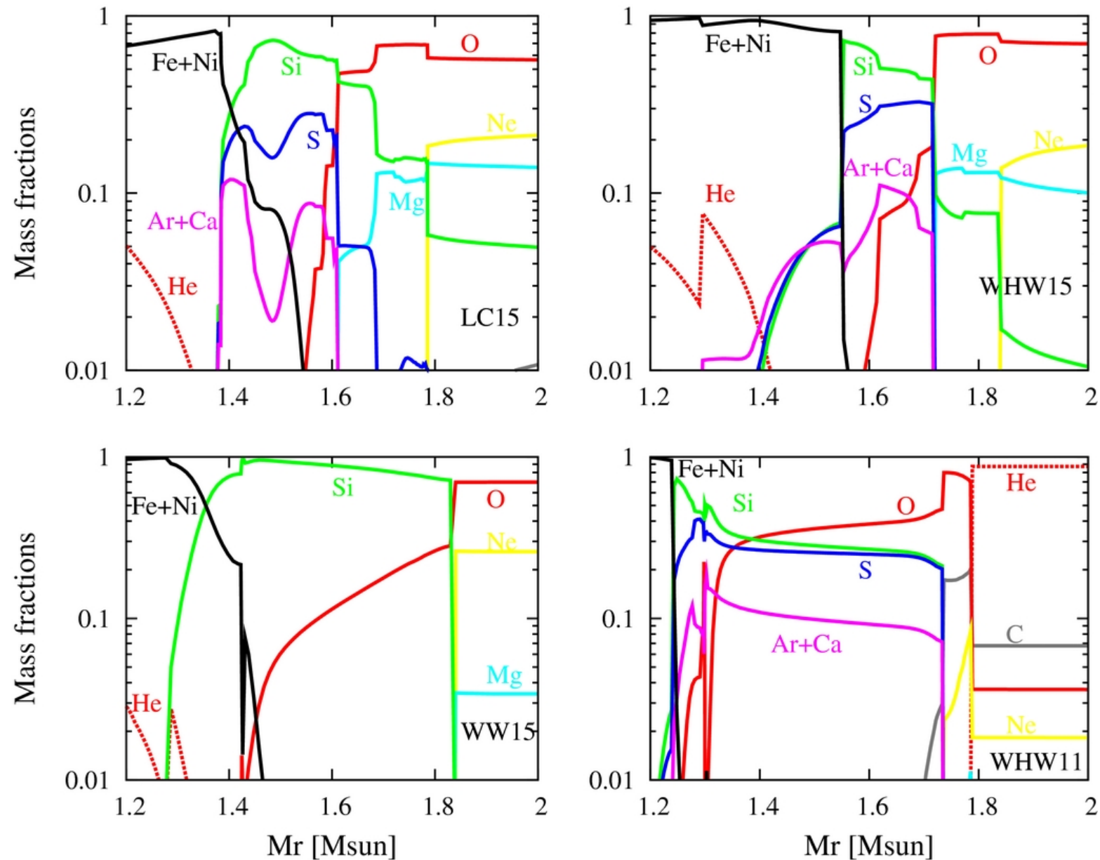
Figure 1. from Revisiting Impacts of Nuclear Burning for Reviving Weak Shocks in Neutrino-driven Supernovae Nakamura et al. 2014 ApJ 782 91 doi:10.1088/0004-637X/782/2/91 https://dx.doi.org/10.1088/0004-637X/782/2/91 © 2014. The American Astronomical Society. All rights reserved.
