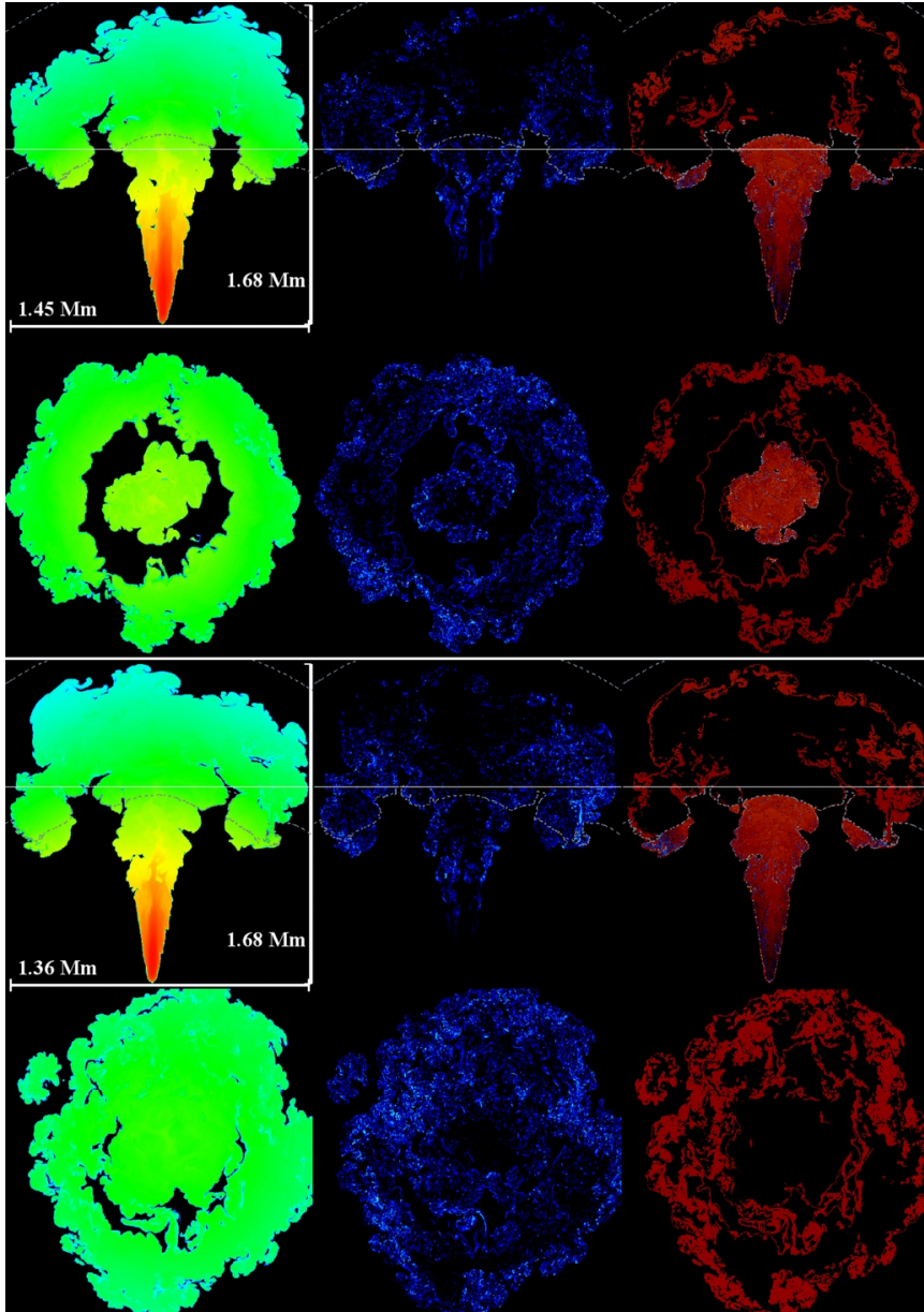
Figure 8. from The Deflagration Stage of Chandrasekhar Mass Models for Type Ia Supernovae. I. Early Evolution Malone et al. 2014 ApJ 782 11 doi:10.1088/0004-637X/782/1/11 https://dx.doi.org/10.1088/0004-637X/782/1/11 © 2014. The American Astronomical Society. All rights reserved.
