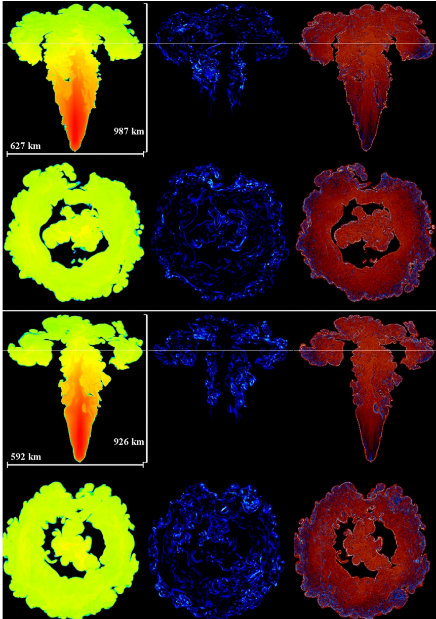
Figure 7. from The Deflagration Stage of Chandrasekhar Mass Models for Type Ia Supernovae. I. Early Evolution Malone et al. 2014 ApJ 782 11 doi:10.1088/0004-637X/782/1/11 https://dx.doi.org/10.1088/0004-637X/782/1/11 © 2014. The American Astronomical Society. All rights reserved.
