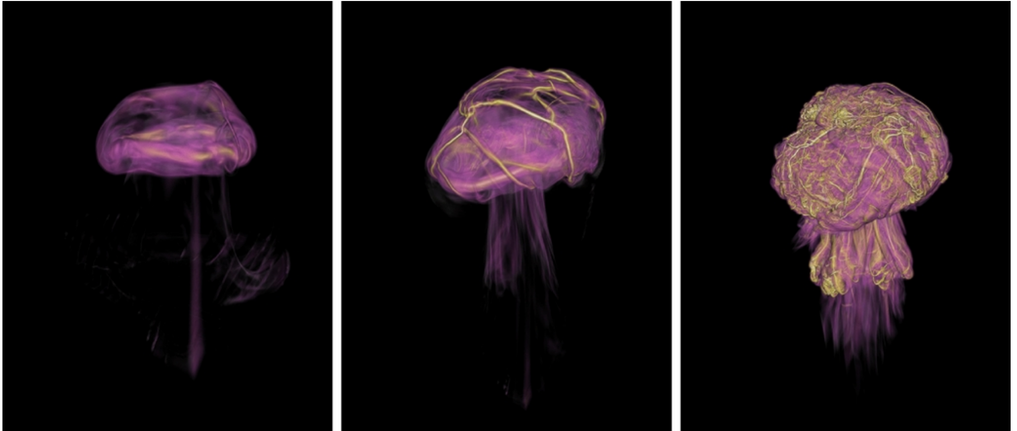
Figure 5. from The Deflagration Stage of Chandrasekhar Mass Models for Type Ia Supernovae. I. Early Evolution Malone et al. 2014 ApJ 782 11 doi:10.1088/0004-637X/782/1/11 https://dx.doi.org/10.1088/0004-637X/782/1/11 © 2014. The American Astronomical Society. All rights reserved.
