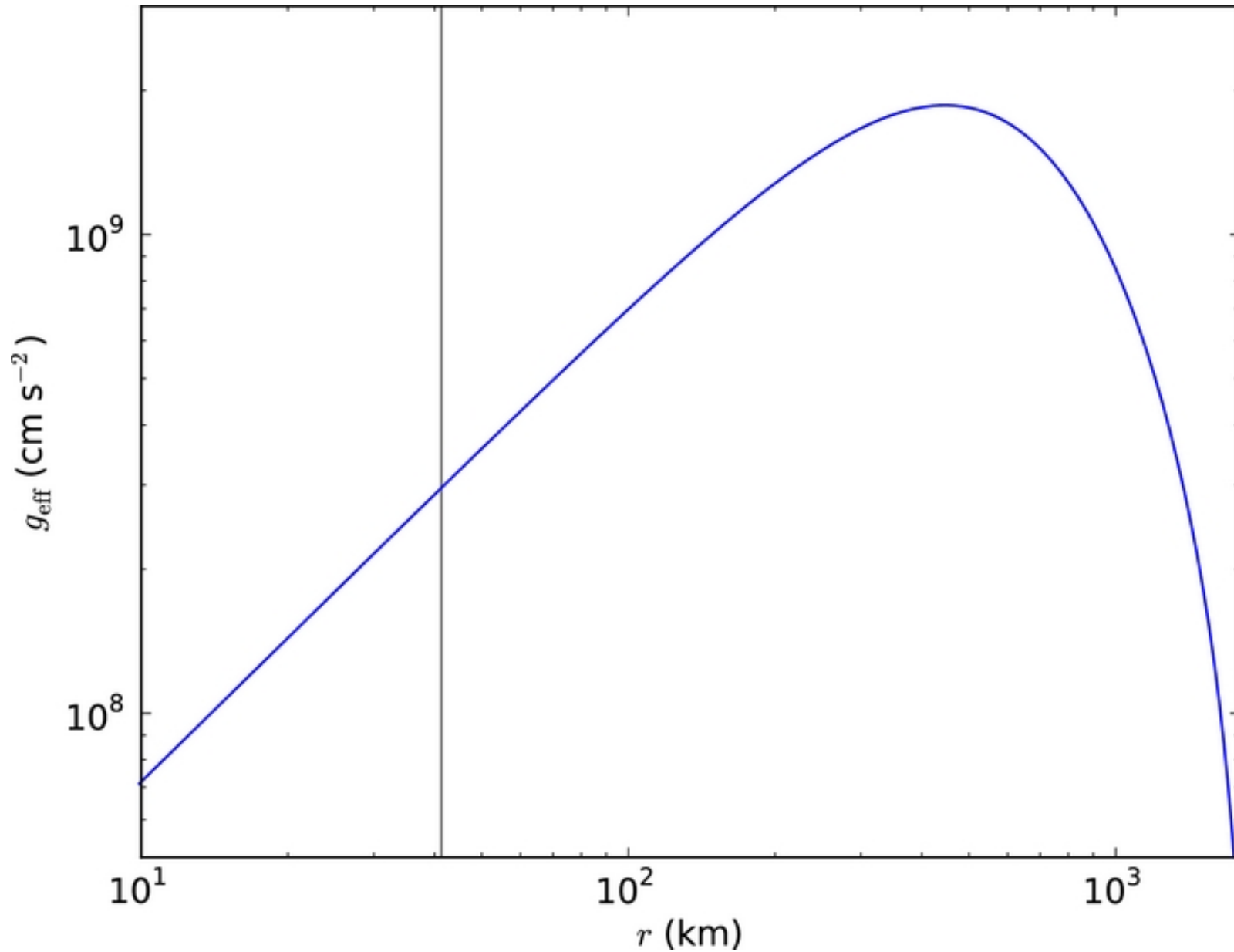
Figure 19. from The Deflagration Stage of Chandrasekhar Mass Models for Type Ia Supernovae. I. Early Evolution Malone et al. 2014 ApJ 782 11 doi:10.1088/0004-637X/782/1/11 https://dx.doi.org/10.1088/0004-637X/782/1/11 © 2014. The American Astronomical Society. All rights reserved.
