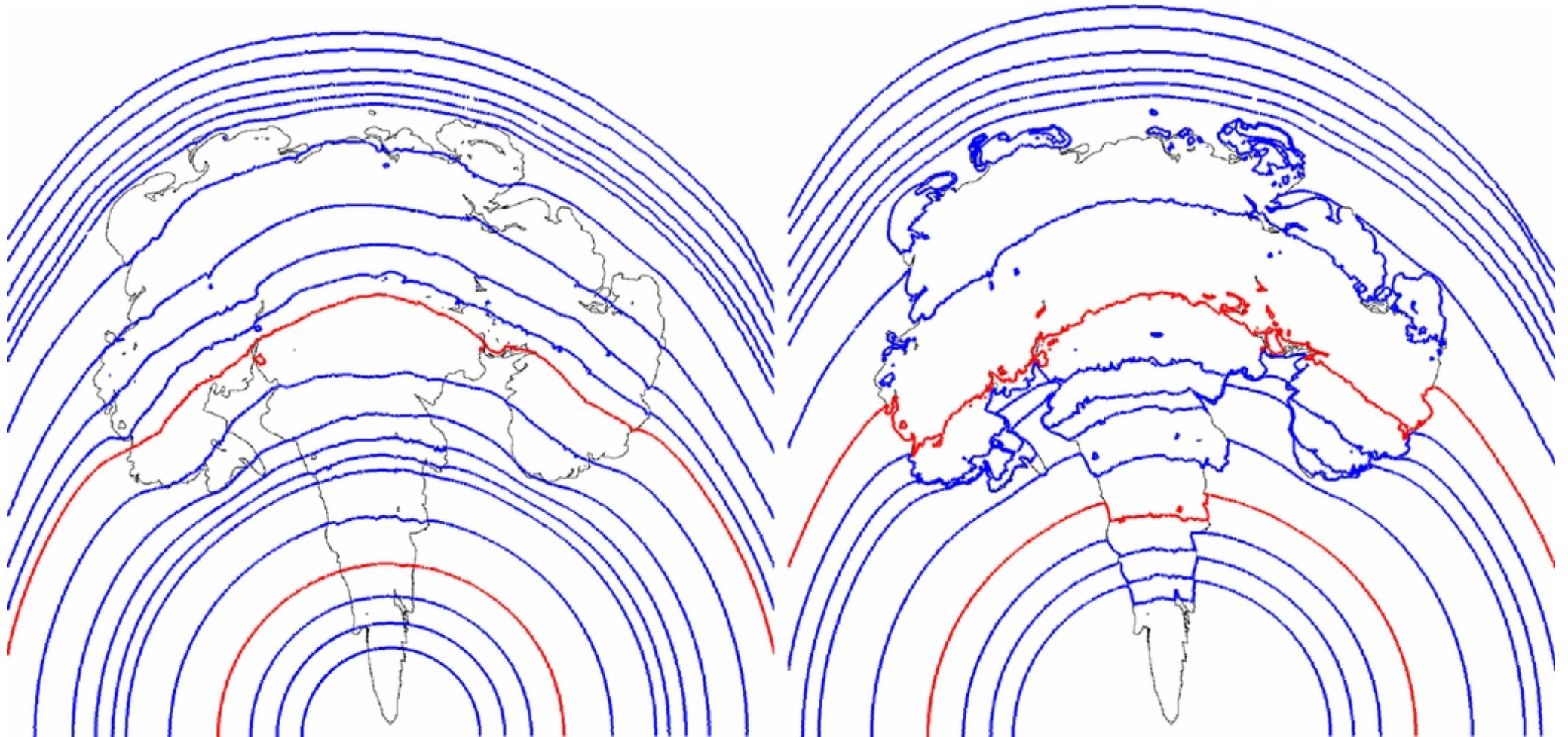
Figure 17. from The Deflagration Stage of Chandrasekhar Mass Models for Type Ia Supernovae. I. Early Evolution Malone et al. 2014 ApJ 782 11 doi:10.1088/0004-637X/782/1/11 https://dx.doi.org/10.1088/0004-637X/782/1/11 © 2014. The American Astronomical Society. All rights reserved.
