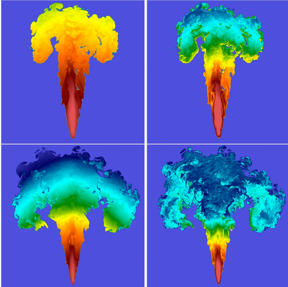
Figure 12. from The Deflagration Stage of Chandrasekhar Mass Models for Type Ia Supernovae. I. Early Evolution Malone et al. 2014 ApJ 782 11 doi:10.1088/0004-637X/782/1/11 https://dx.doi.org/10.1088/0004-637X/782/1/11 © 2014. The American Astronomical Society. All rights reserved.
