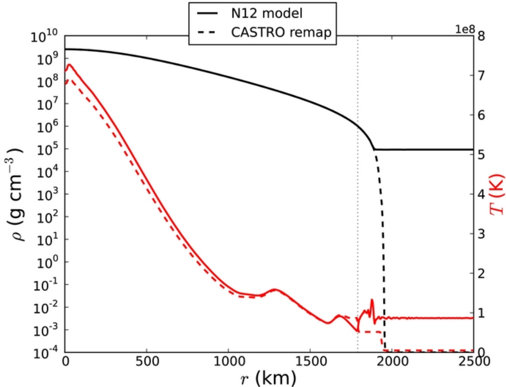
Figure 1. from The Deflagration Stage of Chandrasekhar Mass Models for Type Ia Supernovae. I. Early Evolution Malone et al. 2014 ApJ 782 11 doi:10.1088/0004-637X/782/1/11 https://dx.doi.org/10.1088/0004-637X/782/1/11 © 2014. The American Astronomical Society. All rights reserved.
