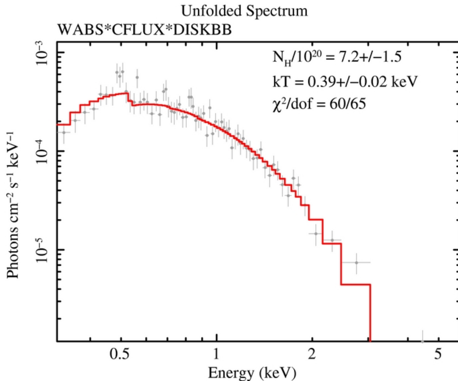
Figure 2. from Discovery of a New Black Hole Transient within 100 (400 pc) of M31* Barnard et al. 2014 ApJ 780 169 doi:10.1088/0004-637X/780/2/169 https://dx.doi.org/10.1088/0004-637X/780/2/169 © 2014. The American Astronomical Society. All rights reserved.
