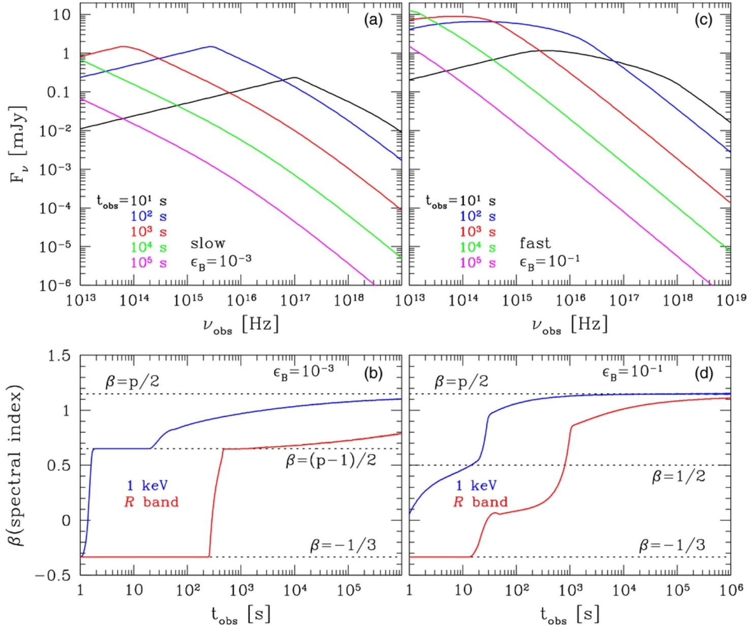
Figure 2. from On the Non-existence of a Sharp Cooling Break in Gamma-Ray Burst Afterglow Spectra Uhm & Zhang 2014 ApJ 780 82 doi:10.1088/0004-637X/780/1/82 https://dx.doi.org/10.1088/0004-637X/780/1/82
