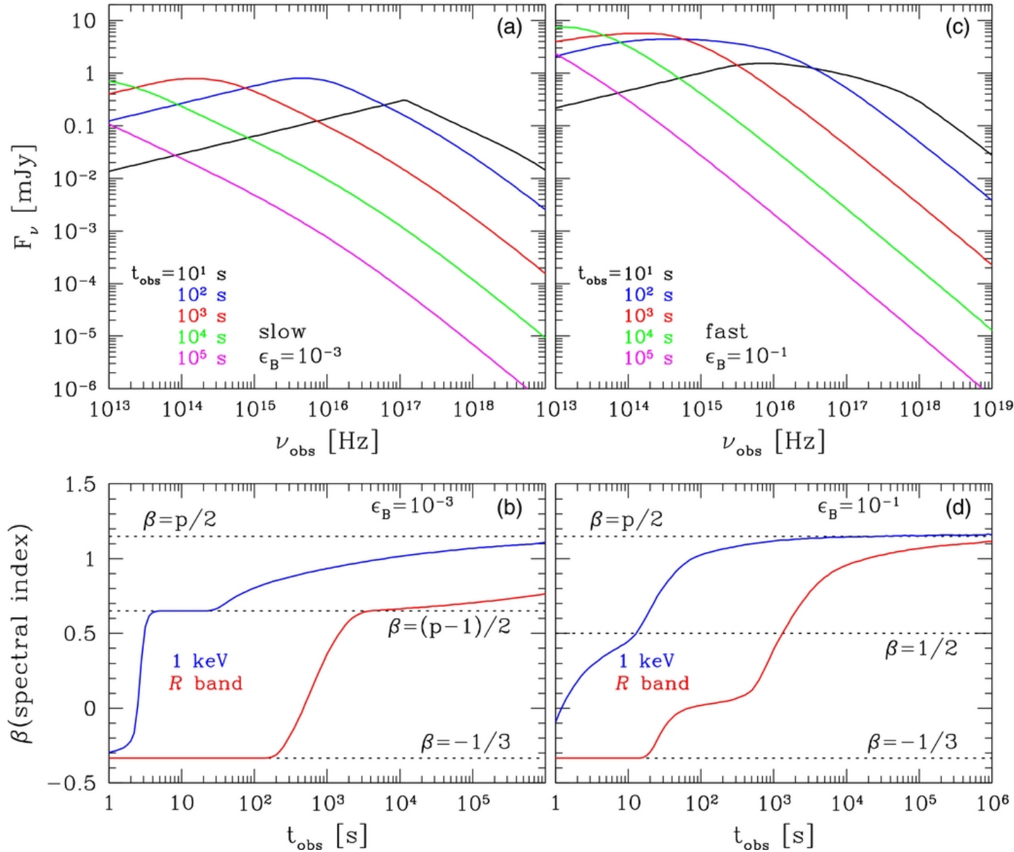
Figure 1. from On the Non-existence of a Sharp Cooling Break in Gamma-Ray Burst Afterglow Spectra Uhm & Zhang 2014 ApJ 780 82 doi:10.1088/0004-637X/780/1/82 https://dx.doi.org/10.1088/0004-637X/780/1/82 © 2014. The American Astronomical Society. All rights reserved.
