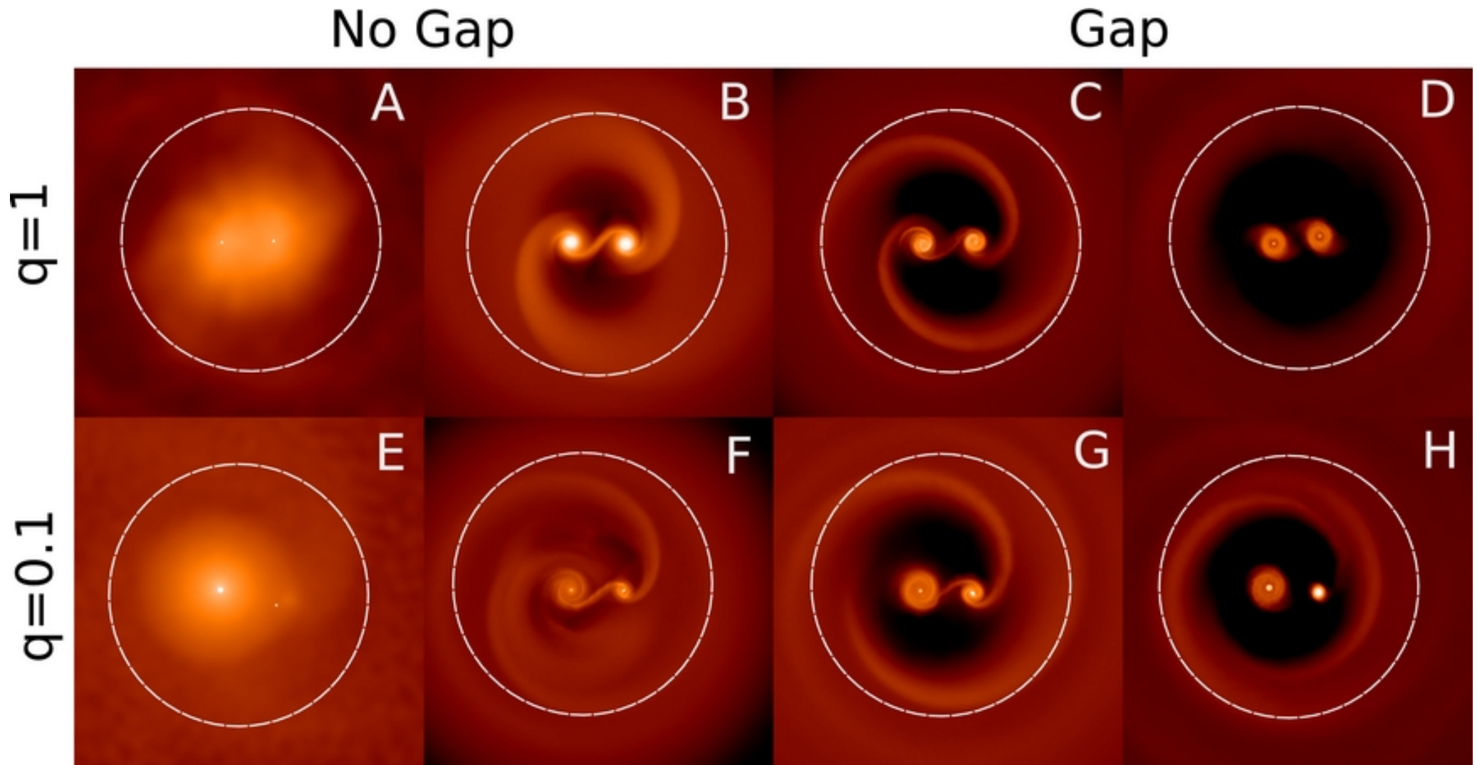
Figure 3. from Binary-Disk Interaction. II. Gap-opening Criteria for Unequal-mass Binaries del Valle & Escala 2014 ApJ 780 84 doi:10.1088/0004-637X/780/1/84 https://dx.doi.org/10.1088/0004-637X/780/1/84 © 2014. The American Astronomical Society. All rights reserved.
