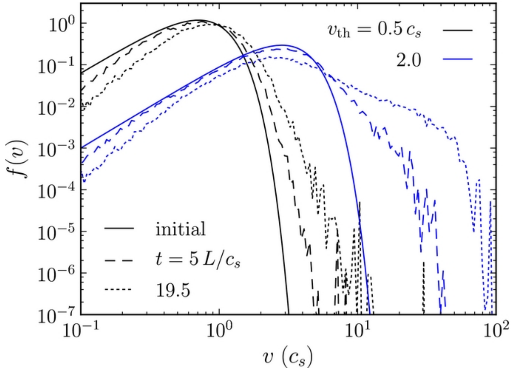
Figure 9. from The Efficiency of Second-order Fermi Acceleration by Weakly Compressible Magnetohydrodynamic Turbulence Lynn et al. 2013 ApJ 777 128 doi:10.1088/0004-637X/777/2/128 https://dx.doi.org/10.1088/0004-637X/777/2/128 © 2013. The American Astronomical Society. All rights reserved.
