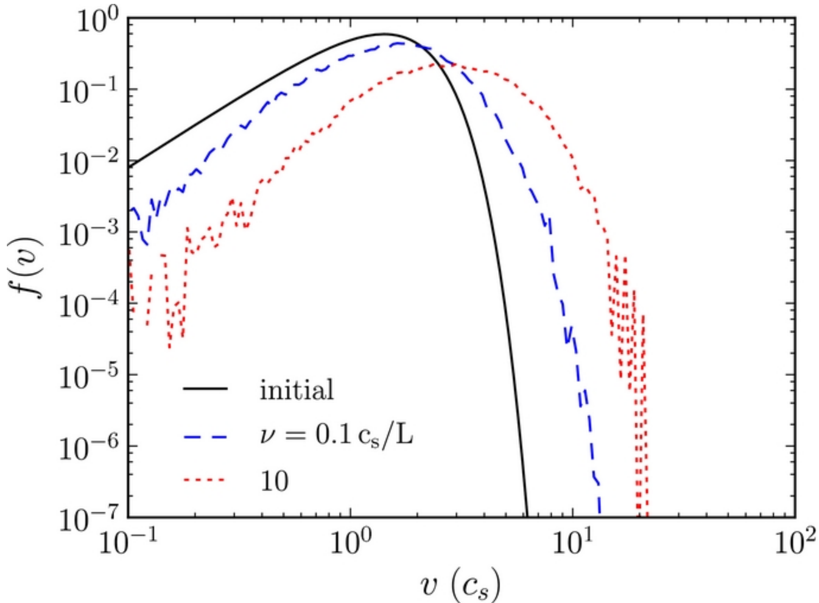
Figure 8. from The Efficiency of Second-order Fermi Acceleration by Weakly Compressible Magnetohydrodynamic Turbulence Lynn et al. 2013 ApJ 777 128 doi:10.1088/0004-637X/777/2/128 https://dx.doi.org/10.1088/0004-637X/777/2/128 © 2013. The American Astronomical Society. All rights reserved.
