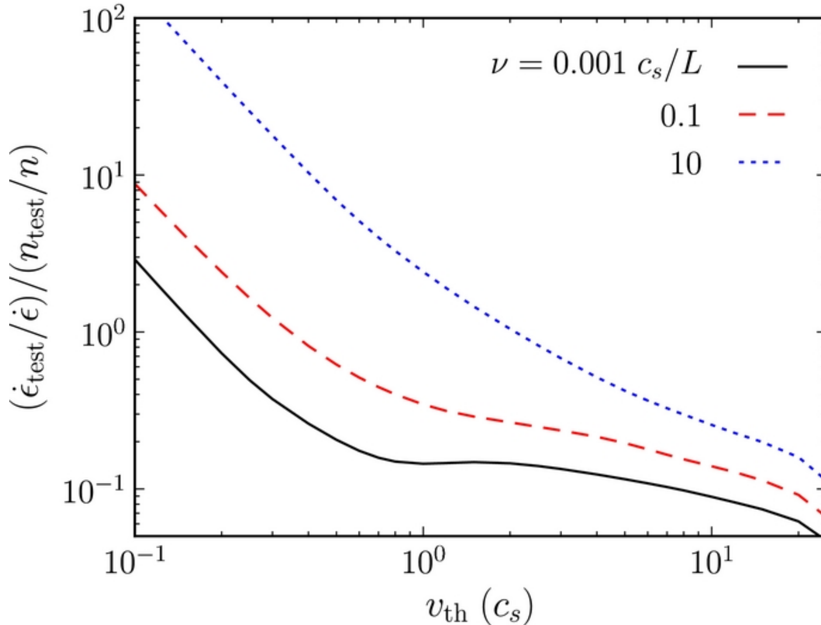
Figure 7. from The Efficiency of Second-order Fermi Acceleration by Weakly Compressible Magnetohydrodynamic Turbulence Lynn et al. 2013 ApJ 777 128 doi:10.1088/0004-637X/777/2/128 https://dx.doi.org/10.1088/0004-637X/777/2/128 © 2013. The American Astronomical Society. All rights reserved.
