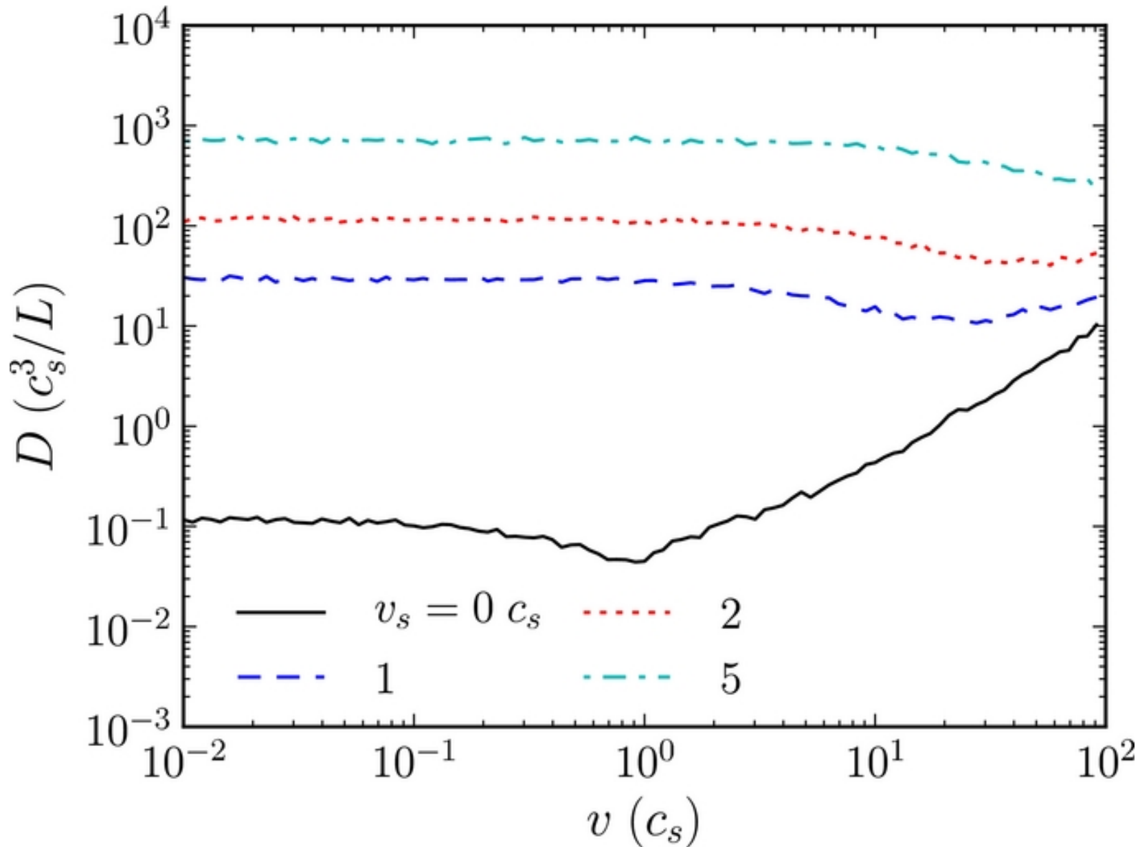
Figure 6. from The Efficiency of Second-order Fermi Acceleration by Weakly Compressible Magnetohydrodynamic Turbulence Lynn et al. 2013 ApJ 777 128 doi:10.1088/0004-637X/777/2/128 https://dx.doi.org/10.1088/0004-637X/777/2/128 © 2013. The American Astronomical Society. All rights reserved.
