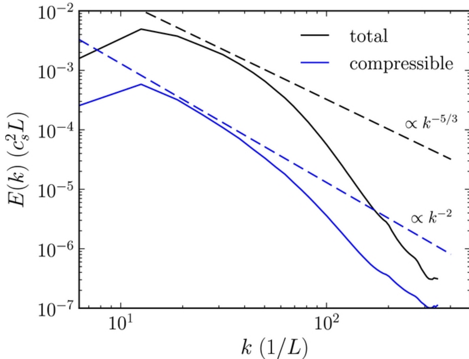
Figure 1. from The Efficiency of Second-order Fermi Acceleration by Weakly Compressible Magnetohydrodynamic Turbulence Lynn et al. 2013 ApJ 777 128 doi:10.1088/0004-637X/777/2/128 https://dx.doi.org/10.1088/0004-637X/777/2/128 © 2013. The American Astronomical Society. All rights reserved.
